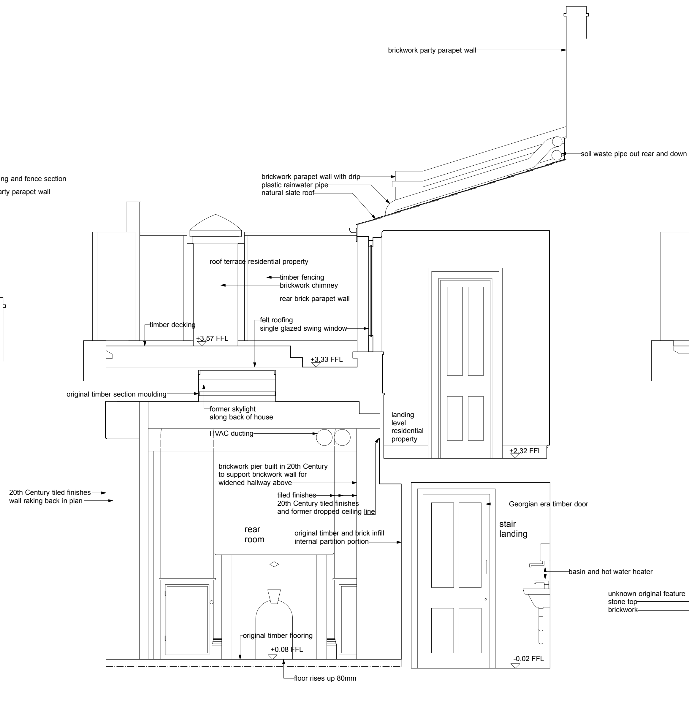
detailed section existing C-C 1:25
