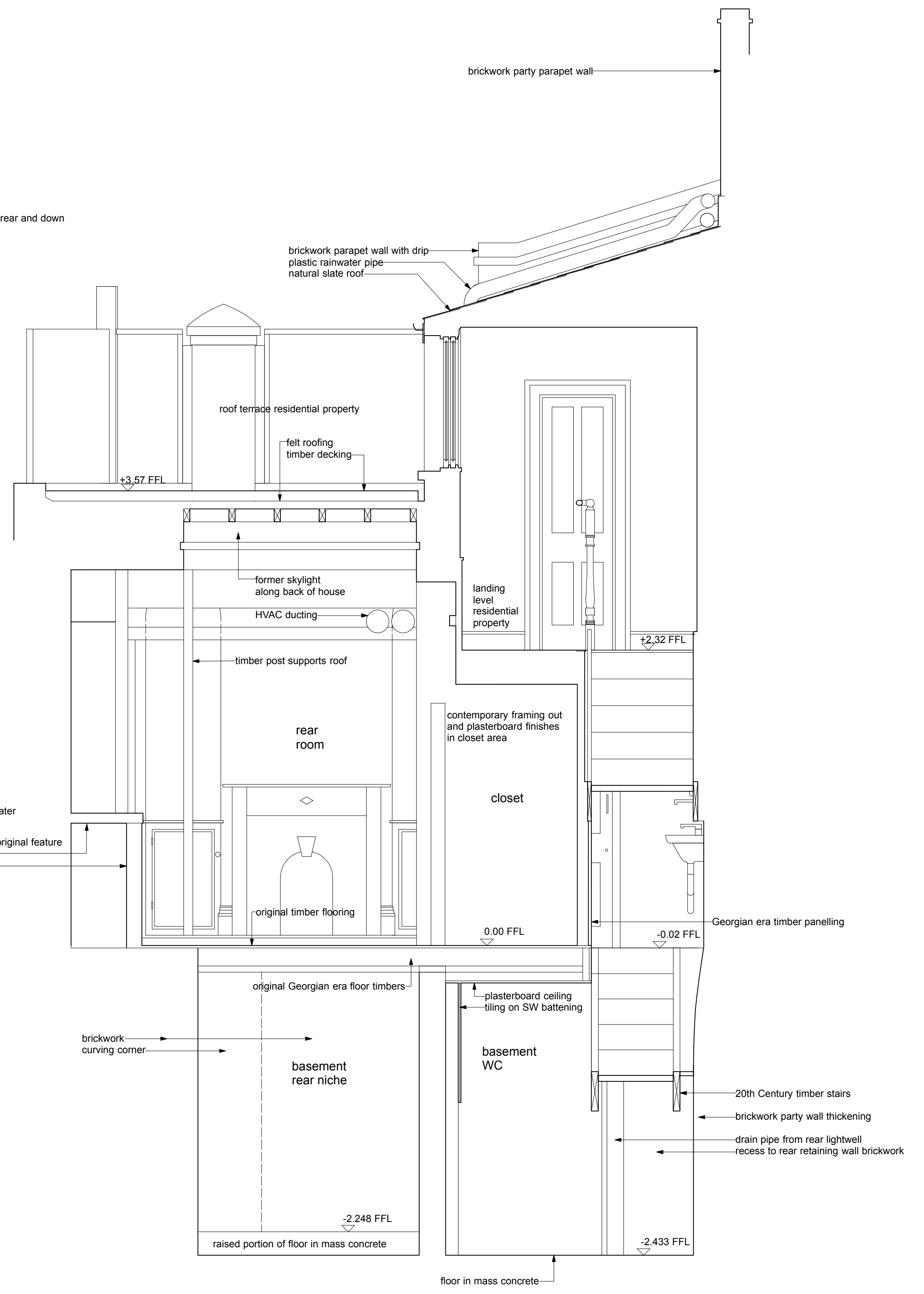
detailed section existing B-B 1:25
