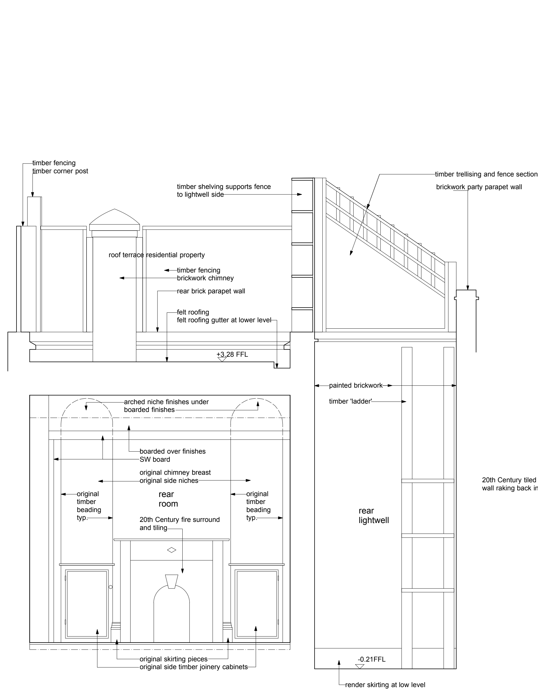
detailed section existing D-D 1:25
