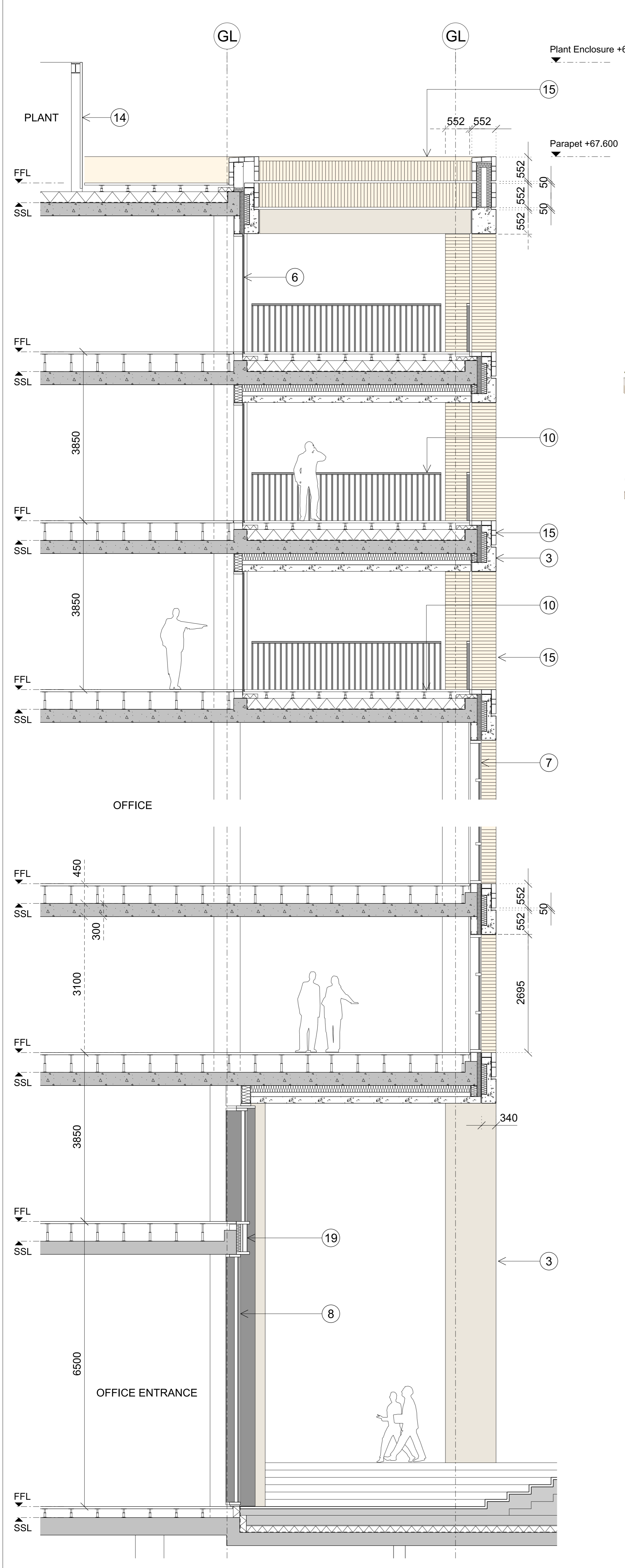
01 Detailed Section - Office entrance, typical office floorplate, upper storey terraces & plant screen
