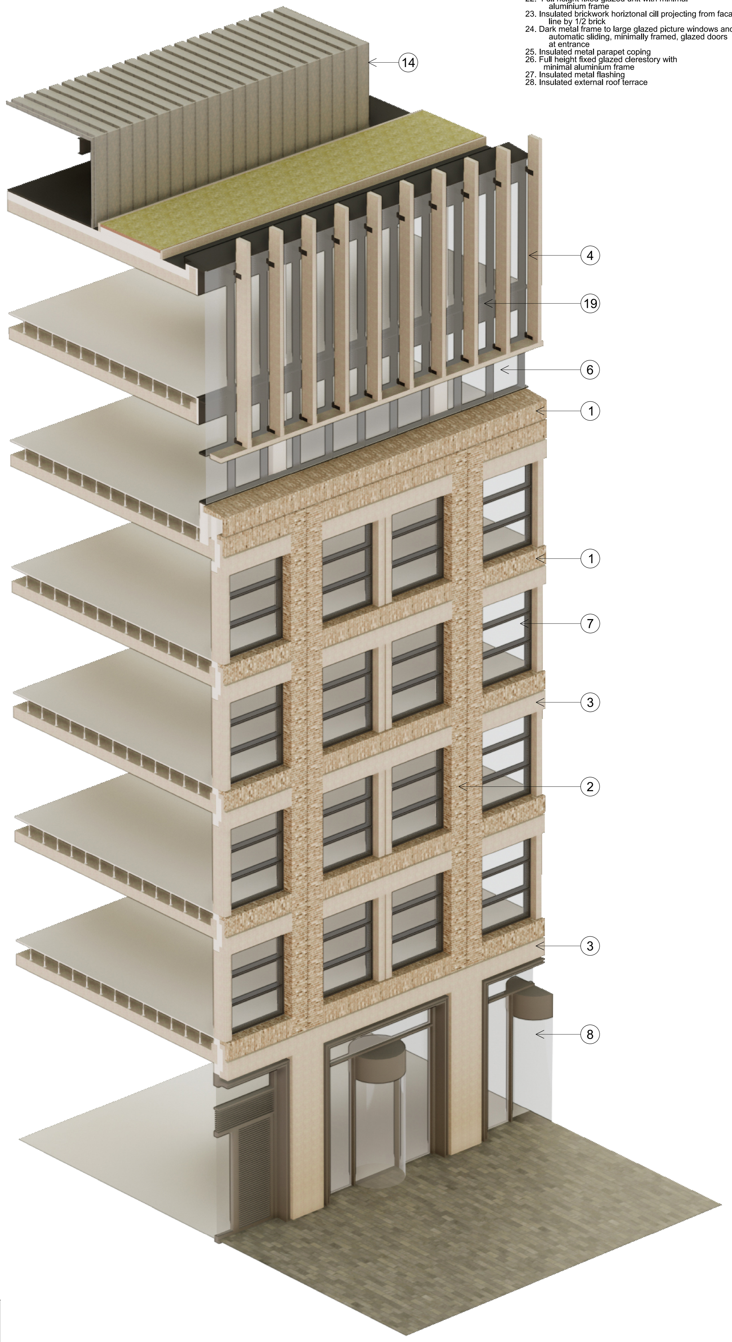
02 Axonometric - Office entrance, typical office parapet, upper storey expression & plant screen
