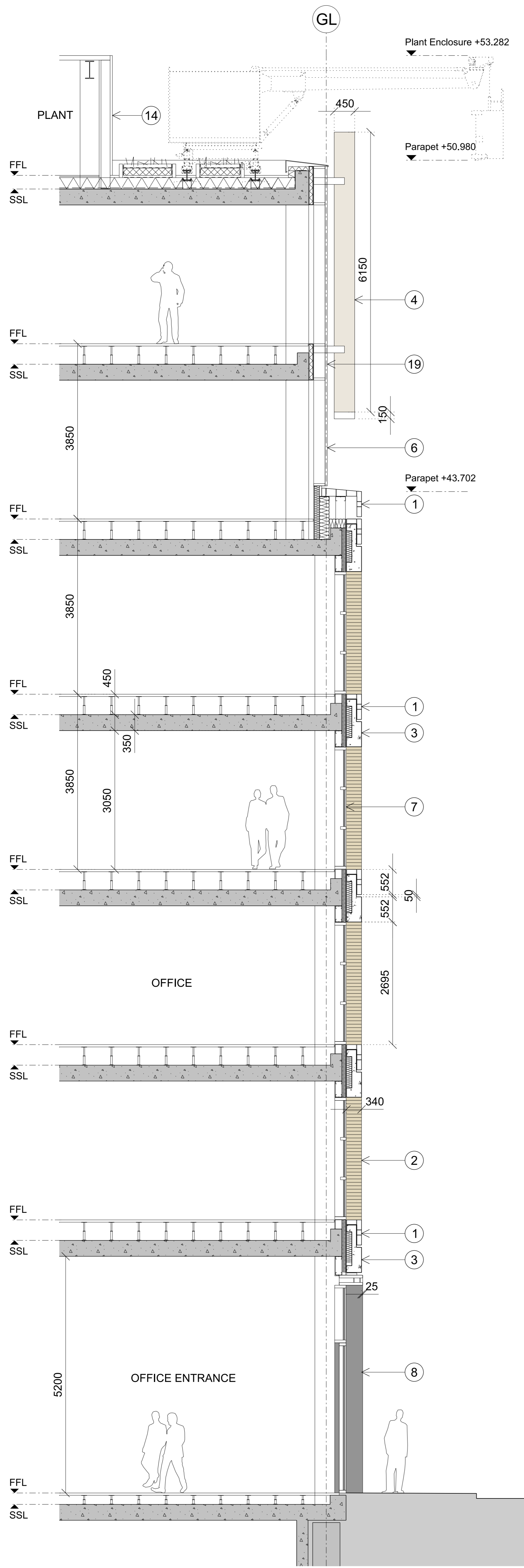
01 Detailed Section - Office entrance, typical office parapet, upper storey expression & plant screen
