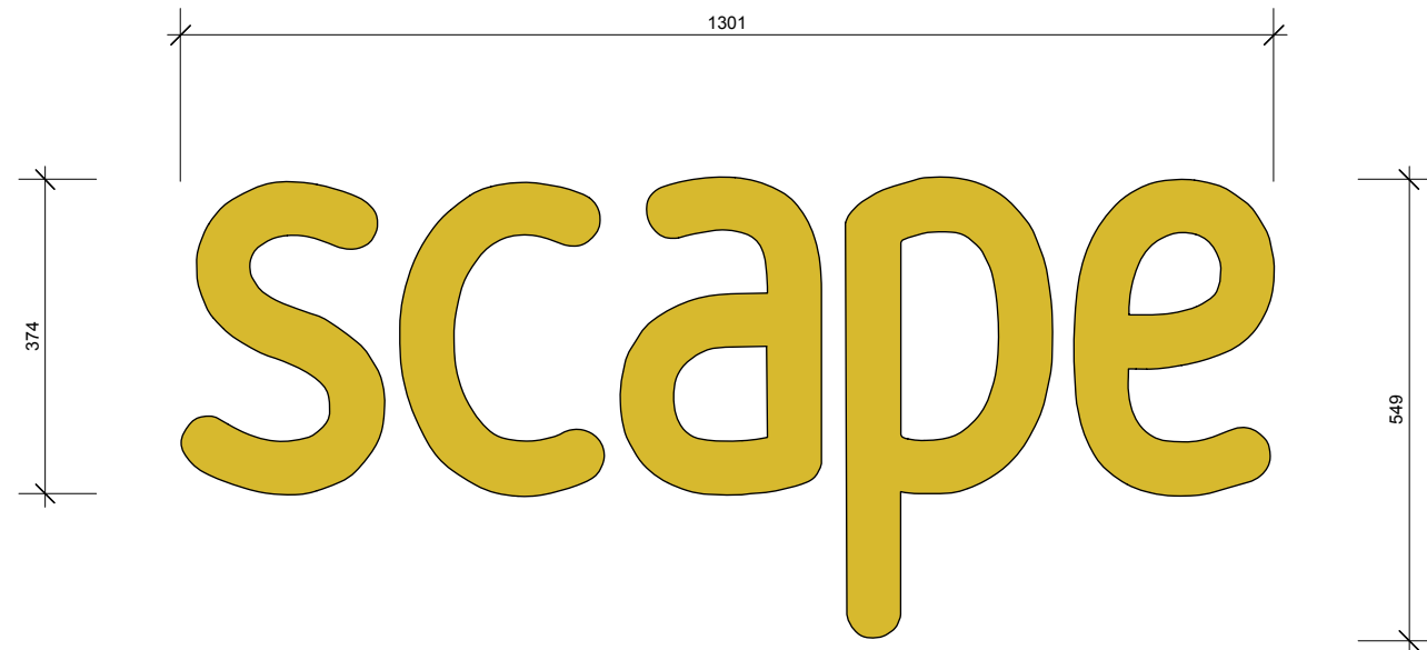
1 Signage Elevation 1:10@A3
