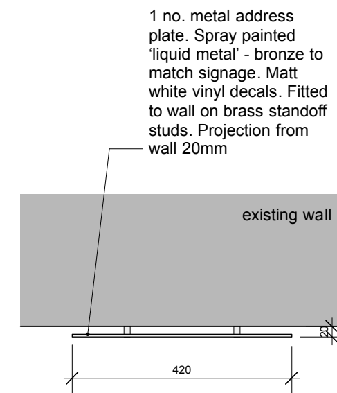
4 Plate Plan 1:10@A3
