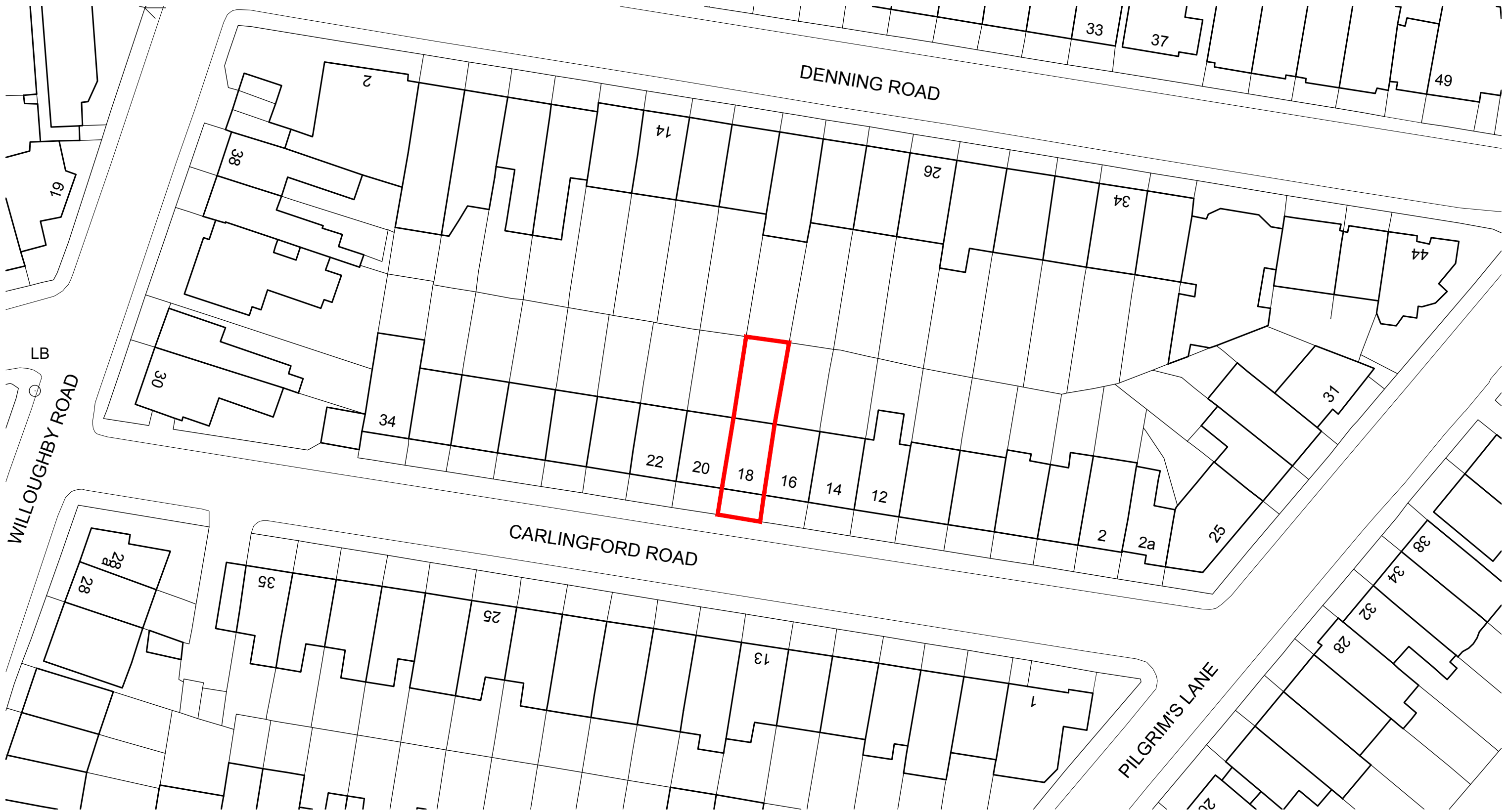
SITE BLOCK PLAN SCALE 1:500
