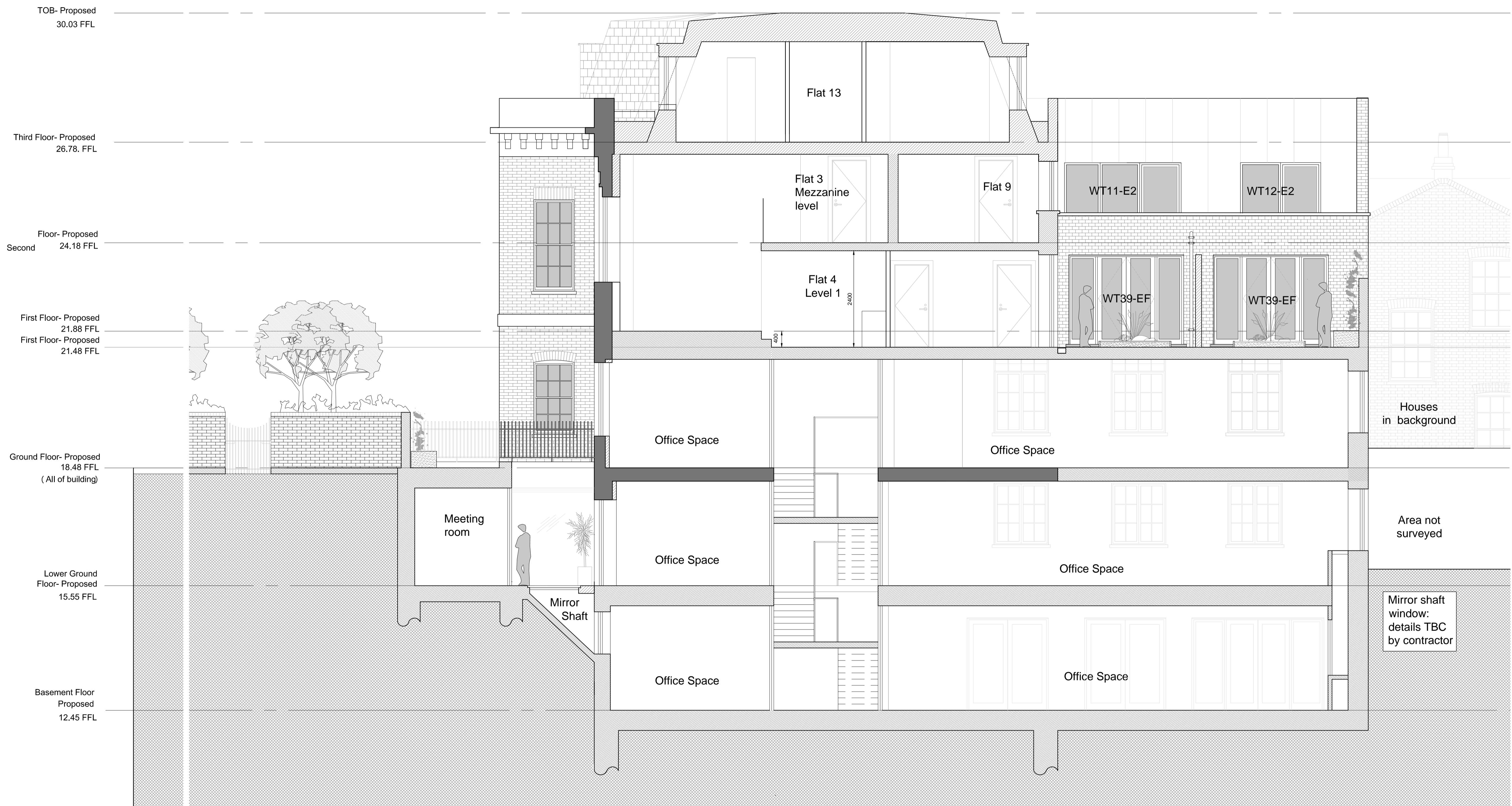
Proposed Section CC Mixed Use Scheme
