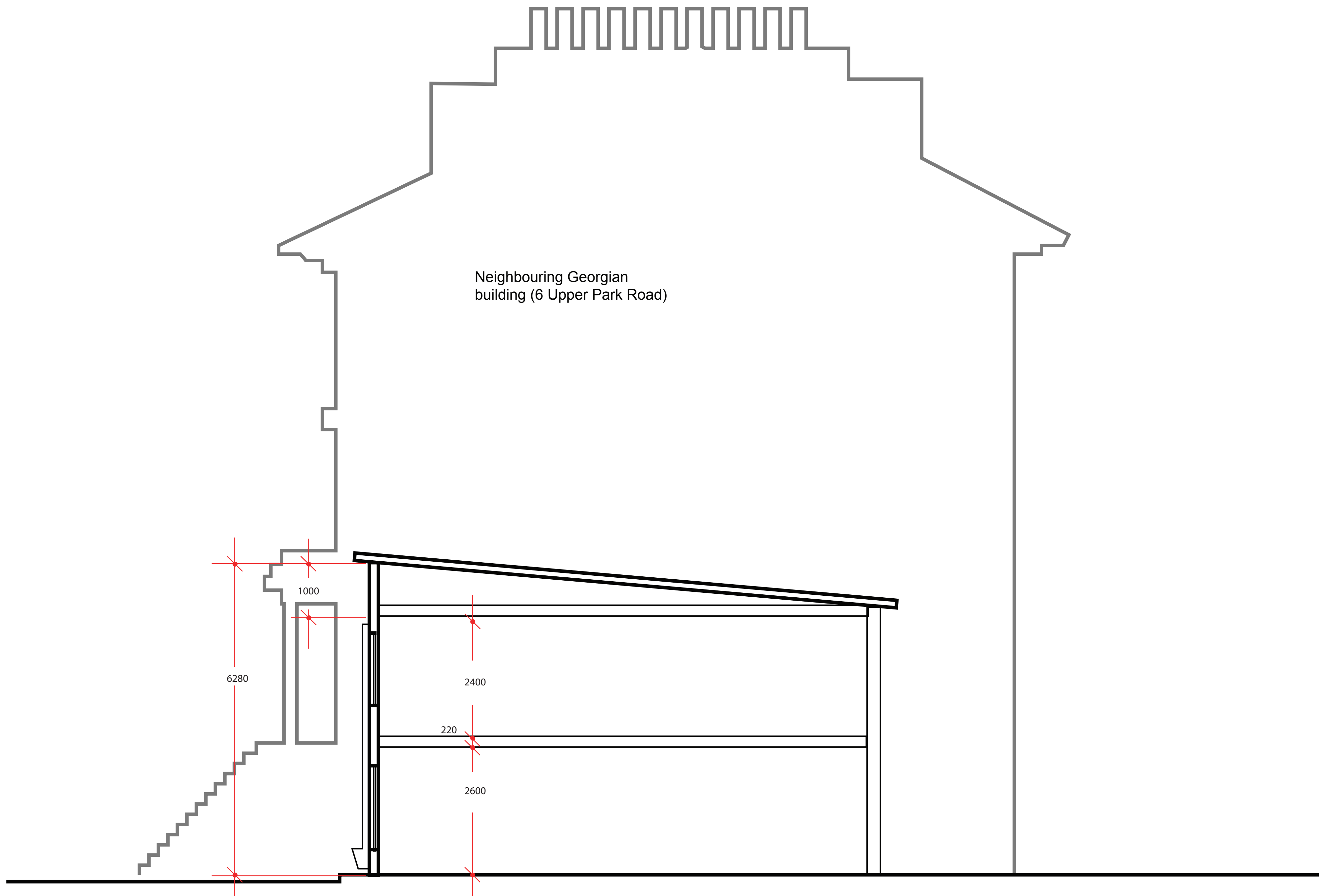
Existing section H:H (see drawings 06 and 29b) through terrace at 4a Upper Park Road Showing comparison of scale between neighbours Drawing 10 - Existing section. Scale 1:50
