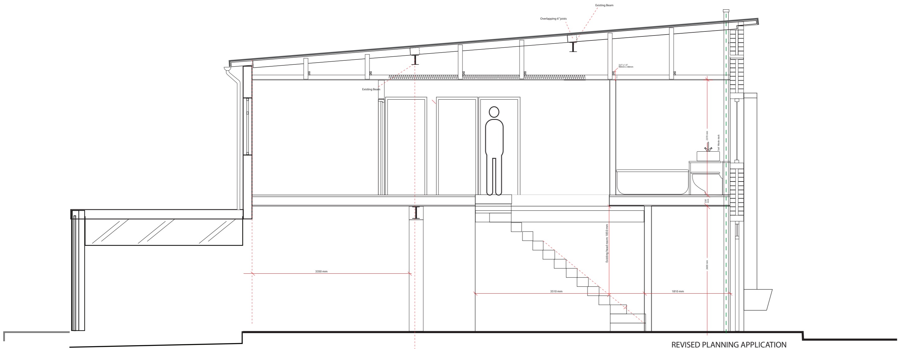
Drawing 23a Existing Section Detail (G-G see Drawing 27b) through terrace at 4a Upper Park Road. SCALE 1:50
