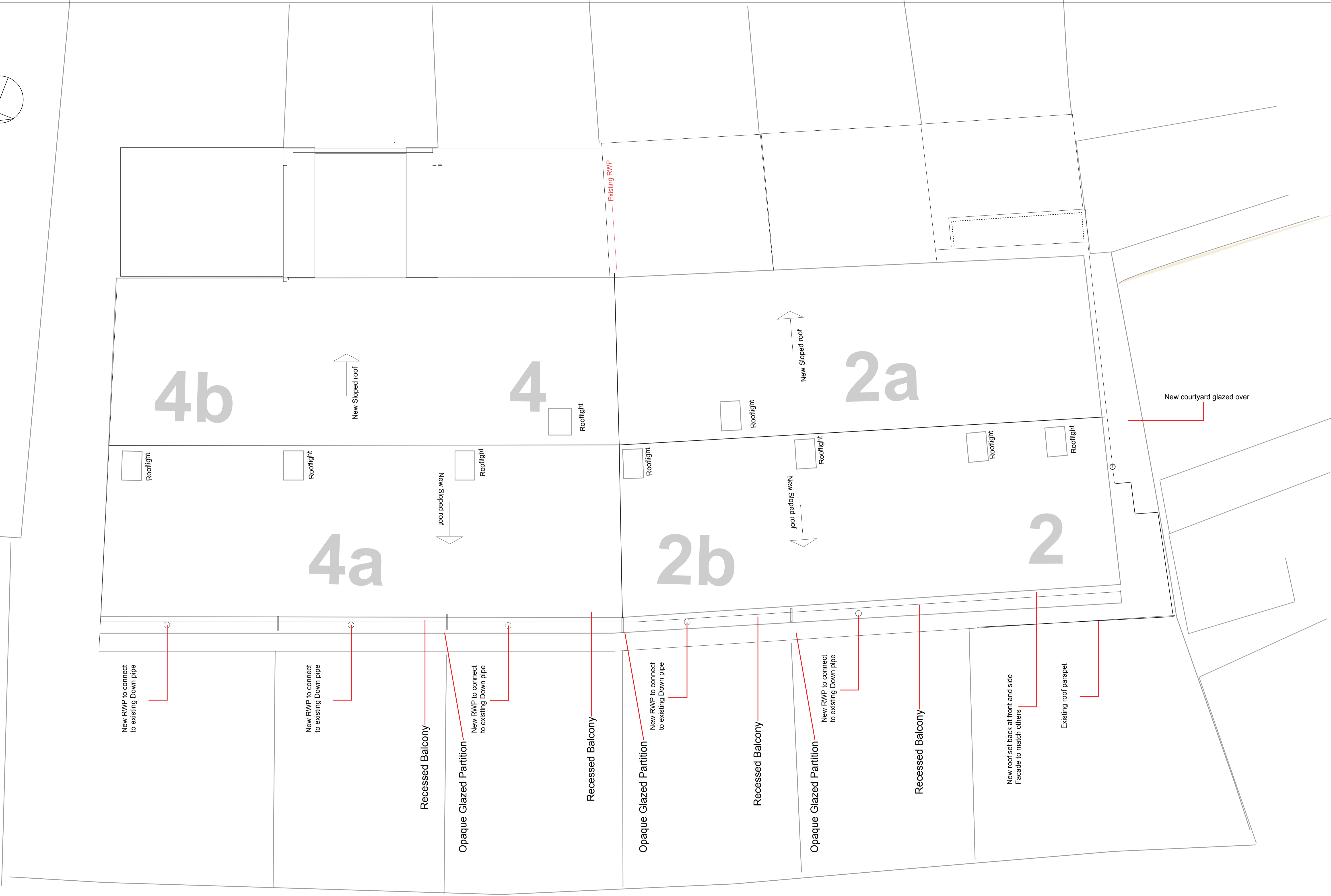
Drawing 014e - Proposed Roof Plan Scale 1:50
