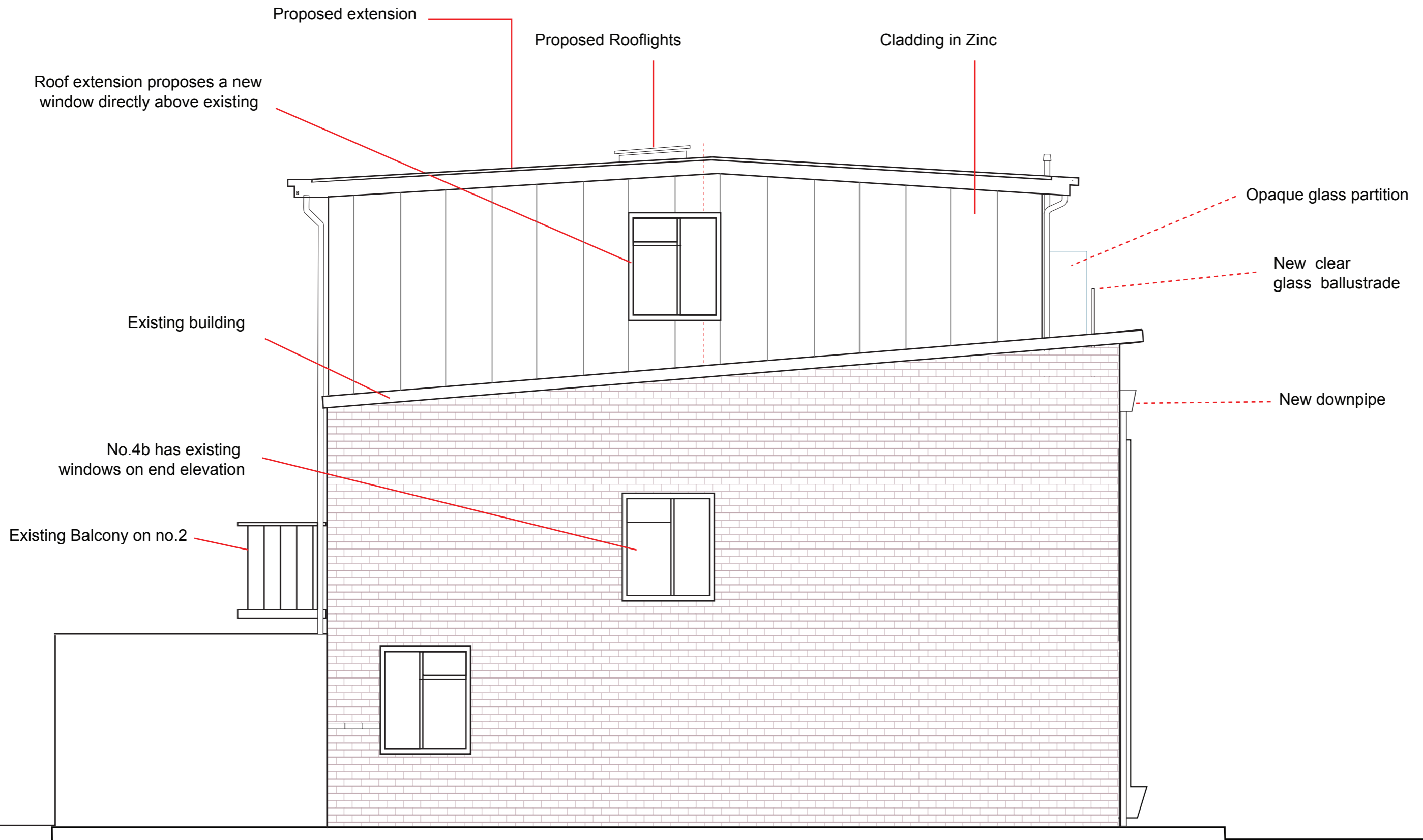
Drawing 13c (East) End Elevation of Terrace 2-4b Upper Park Road
