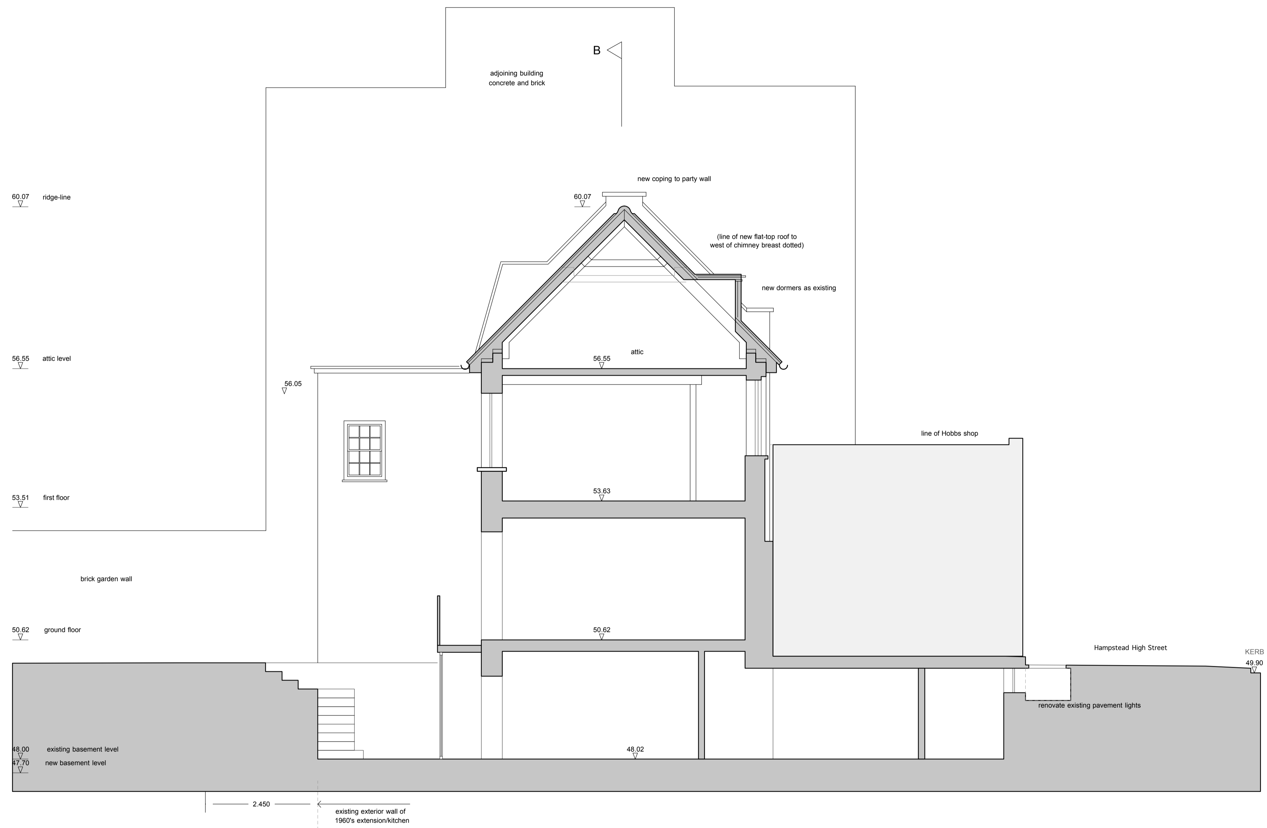
SECTION DD - As Existing
