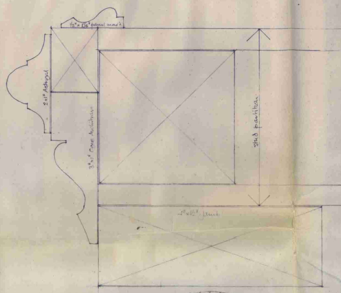
PLAN OF JAMB. F.S.
