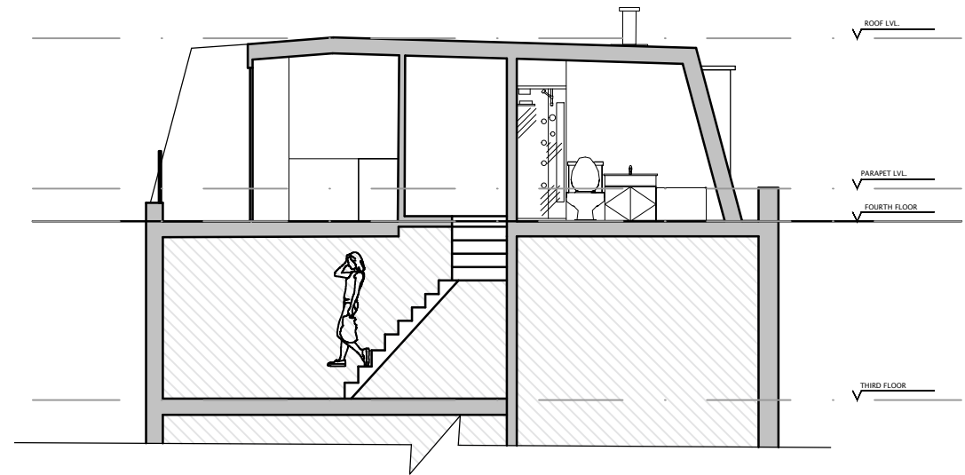
6 SECTION BB PROPOSED 1:100
