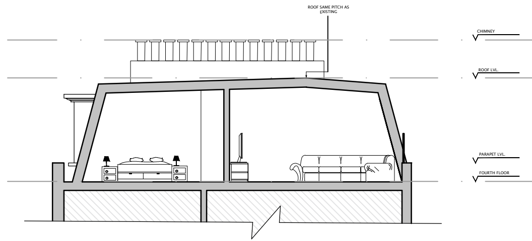
5 SECTION AA PROPOSED 1:100
