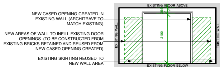
INTERNAL ELEVATION A-A LOWER GROUND FLOOR NEW CASED OPENING
