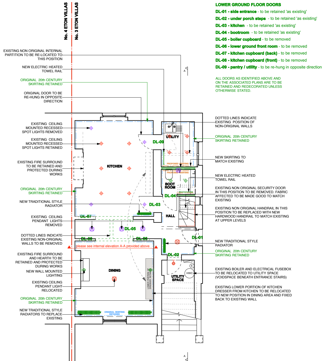
LOWER GROUND PLAN PROPOSED (BASEMENT)
