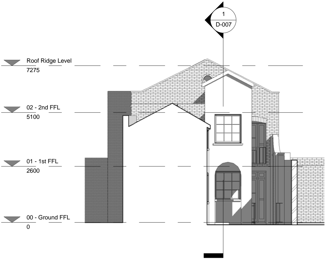
FRONT (SOUTH) ELEVATION 1:100
