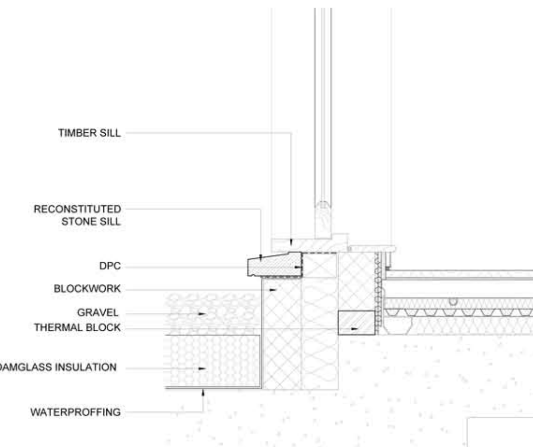
D-D Lightwell Window Details - Head & Sill 1:10 @ A1
