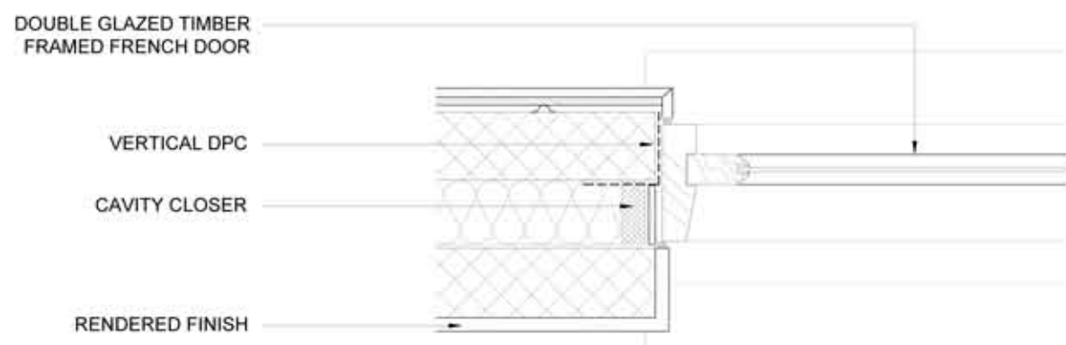
Section A-A French Door / Timber Frame Window Details - Jamb 1:10 @ A1
