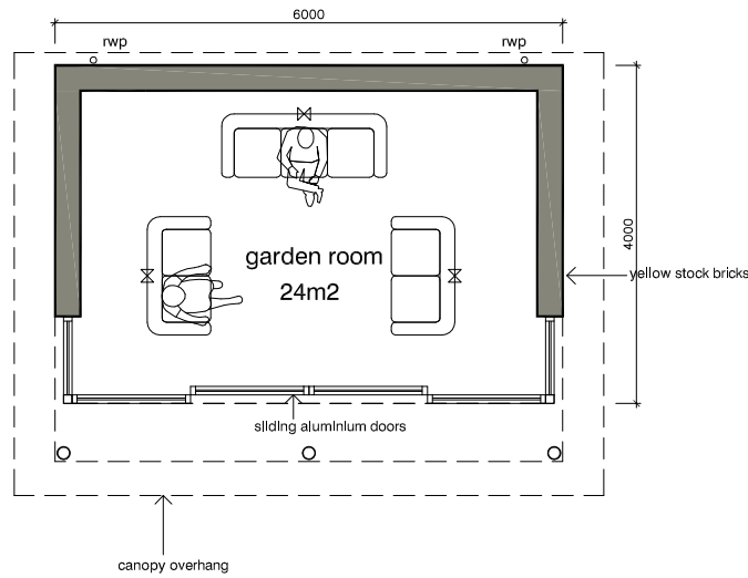
floor plan proposed
