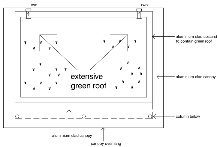
roof plan proposed
