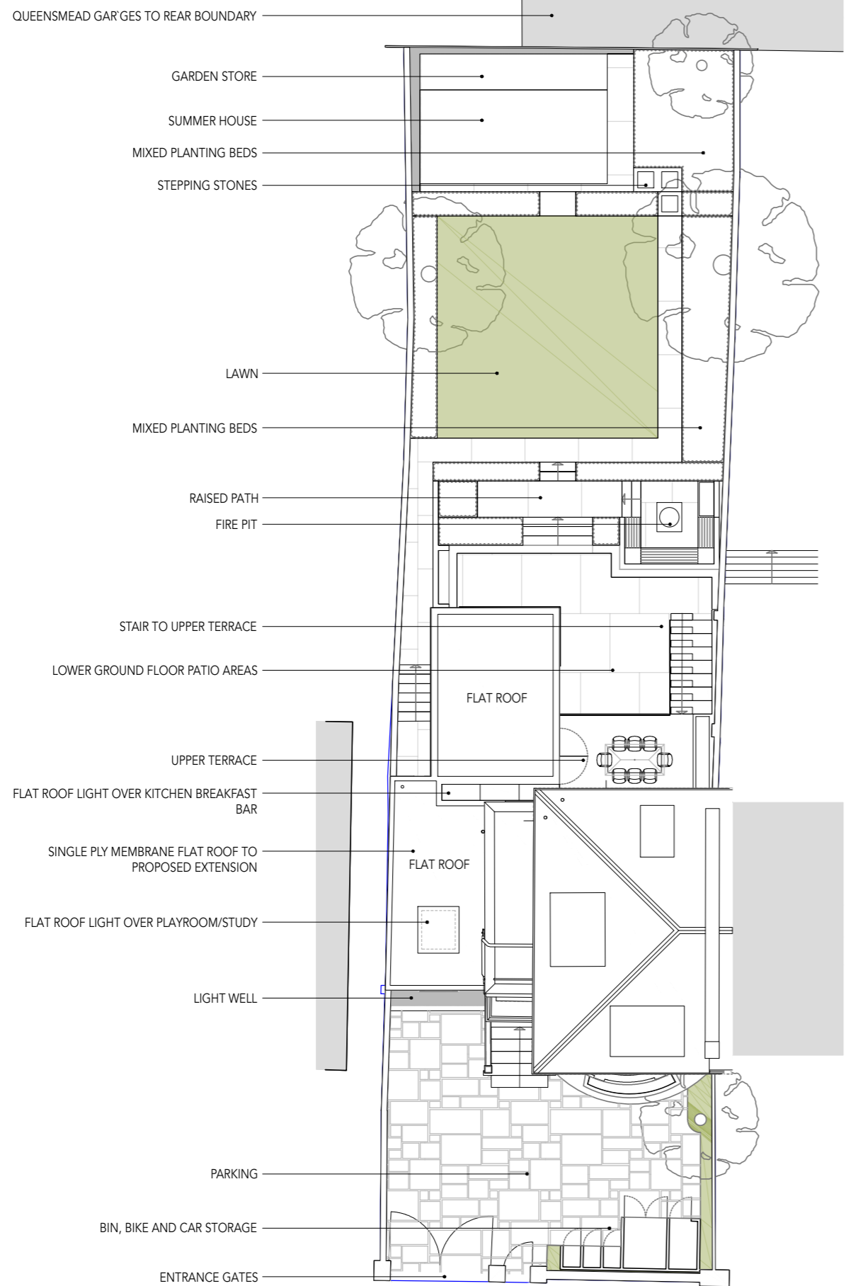
INDICATIVE SUMMER HOUSE AREA 1:100
