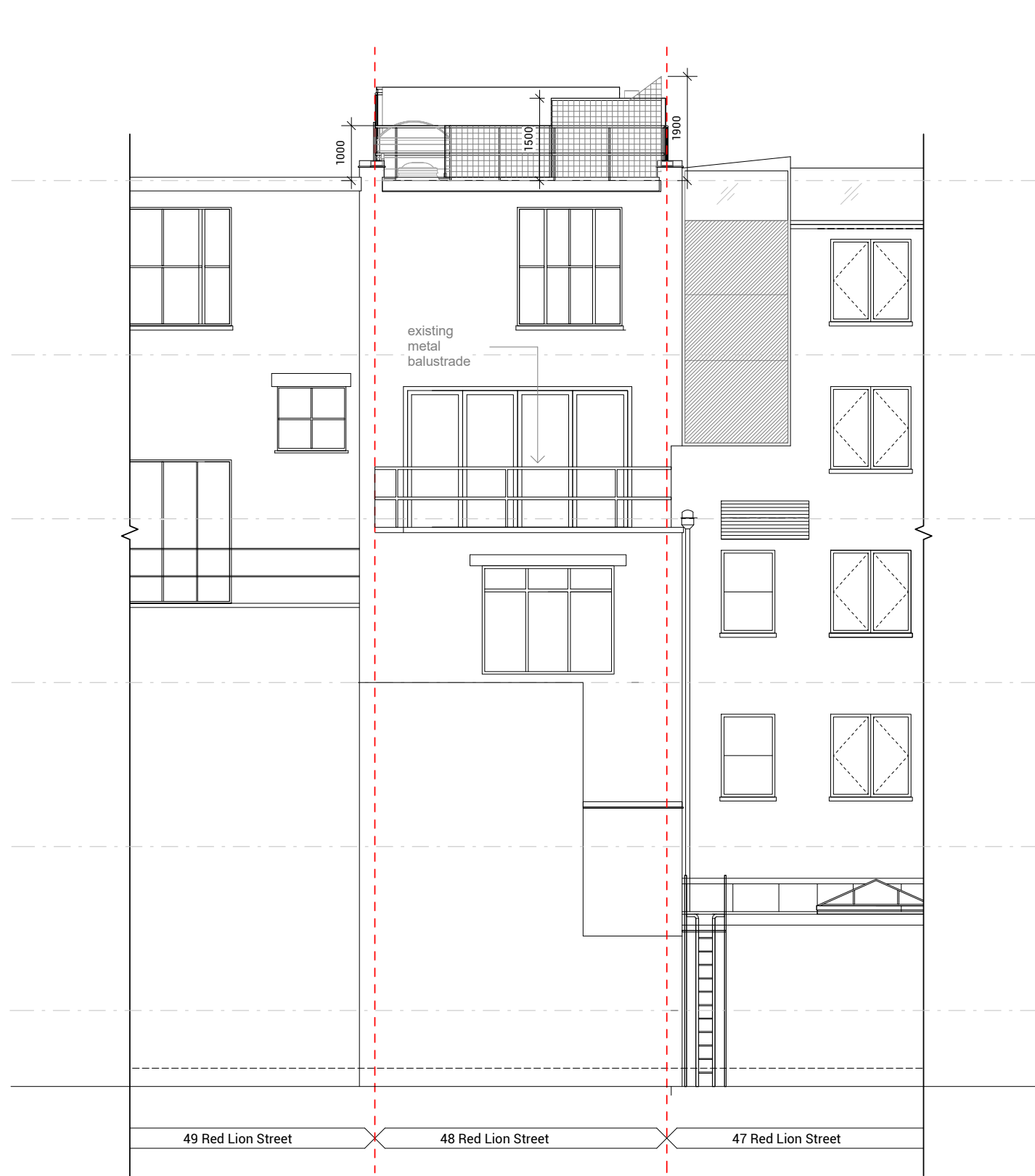
1 Existing Rear Elevation 222-002 1 : 100
