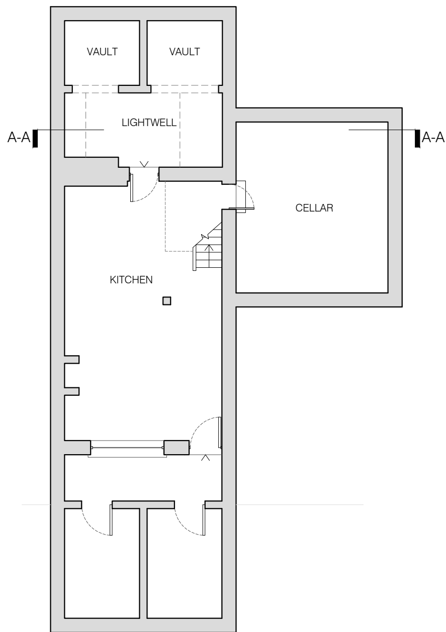
01 EXISTING LOWER GROUND FLOOR PLAN scale 1:100
