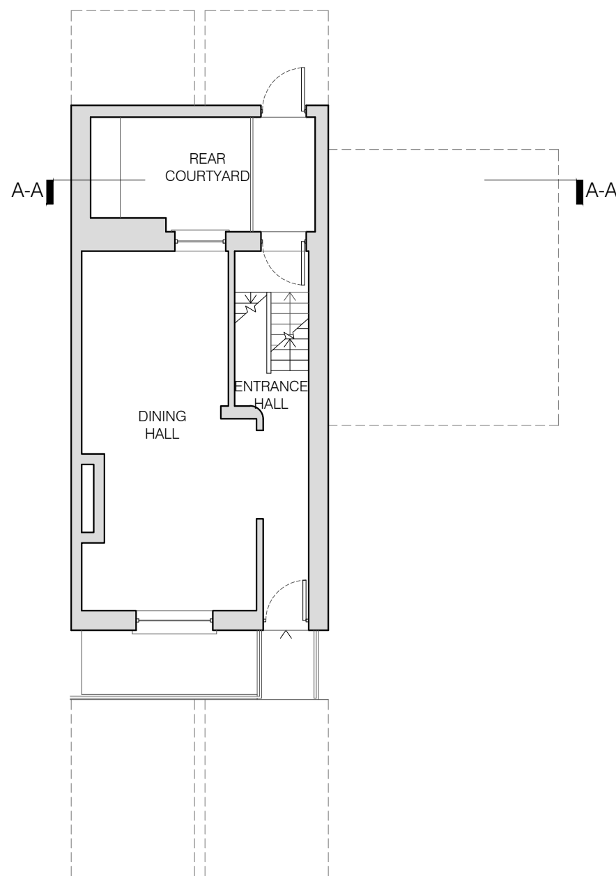
02 EXISTING GROUND FLOOR PLAN scale 1:100
