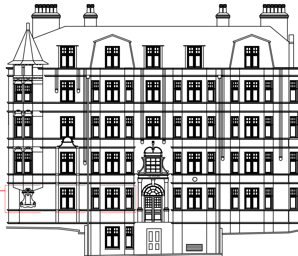
South Elevation
