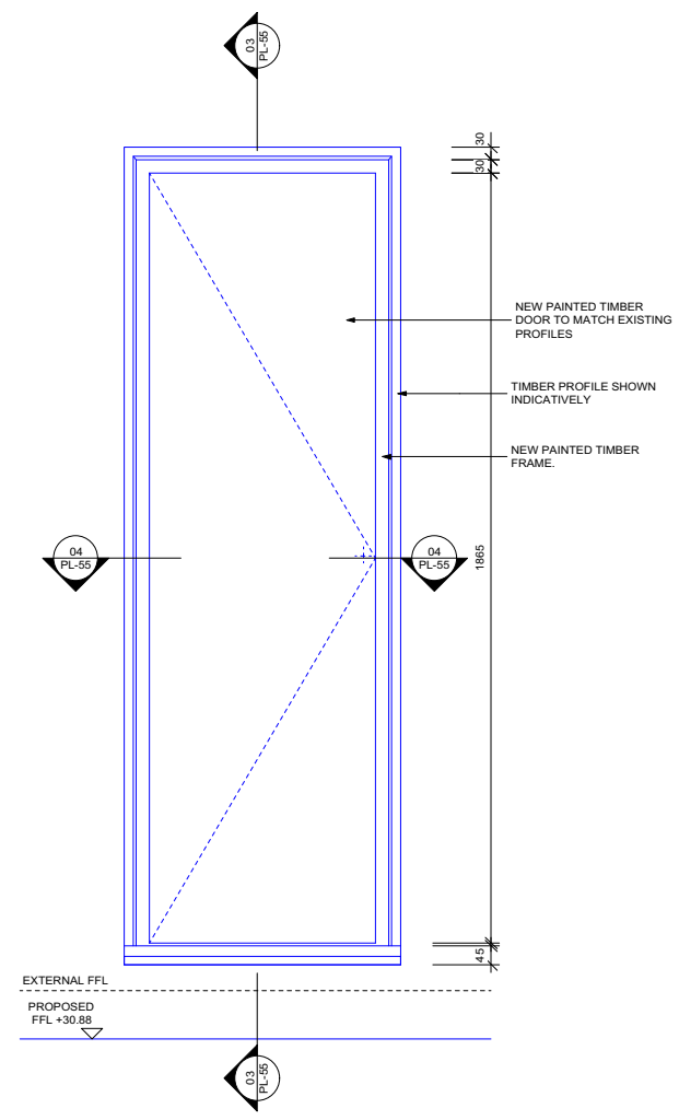
02 DOOR DL18 SCALE 1:10 INTERNAL ELEVATION PL-55
