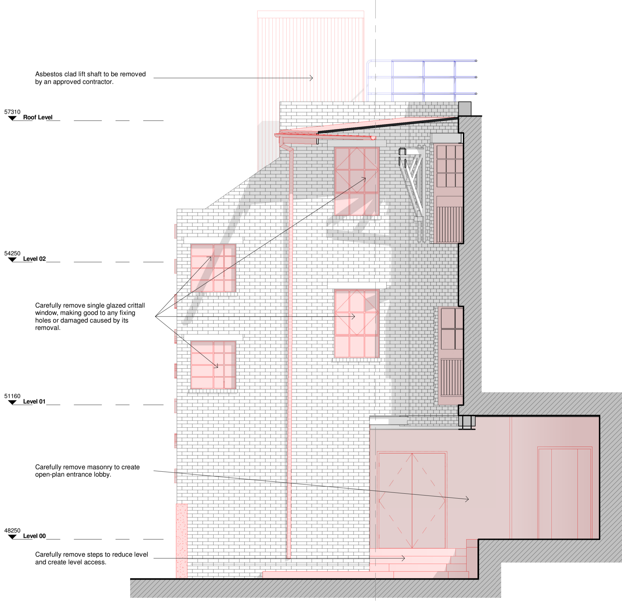
Elevation 2 as Existing
