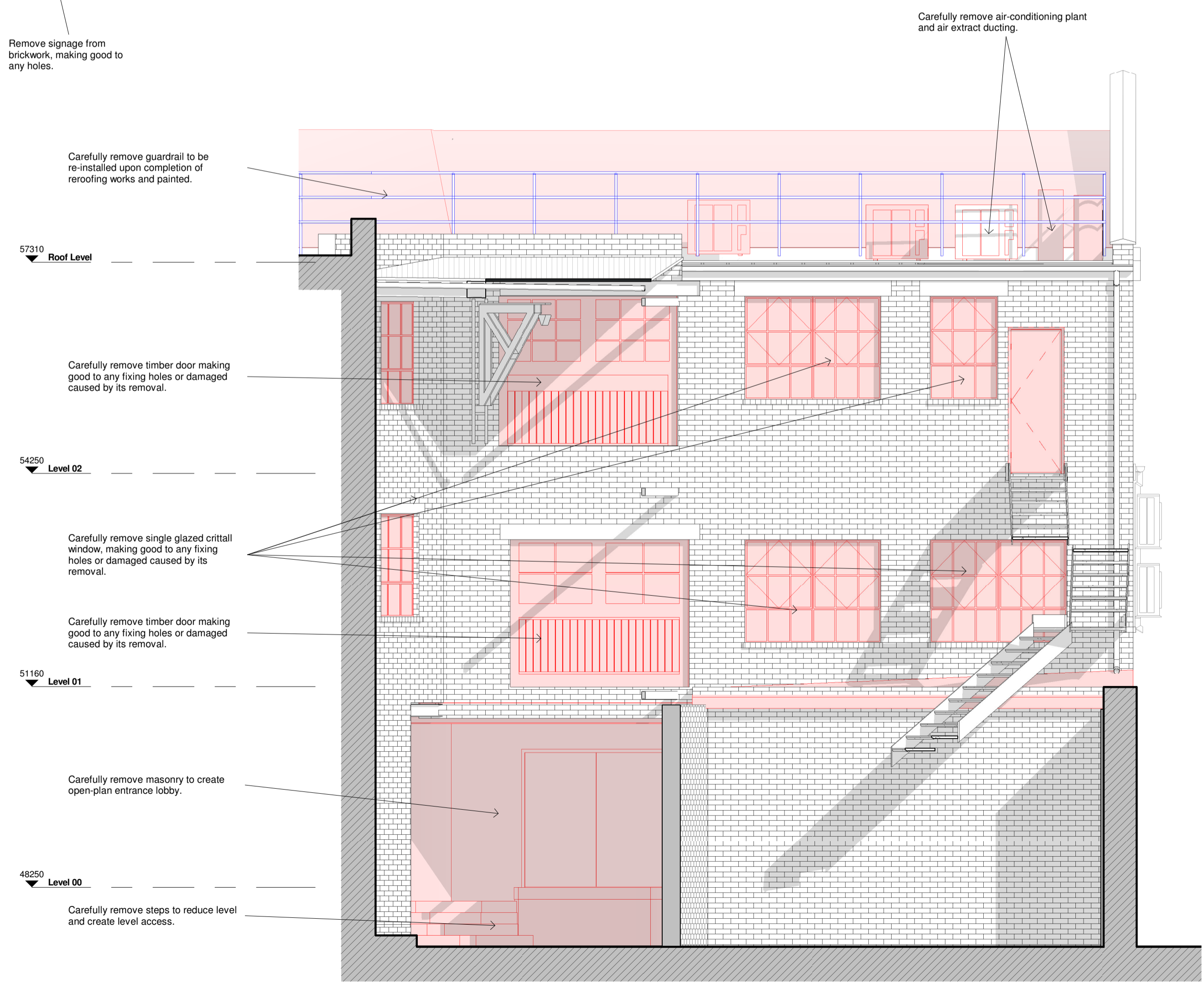
Elevation 3 as Existing
