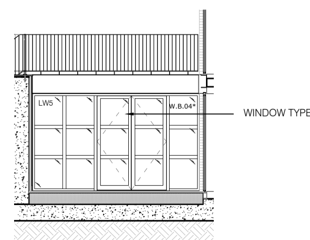
Elevation J Scale 1:100
