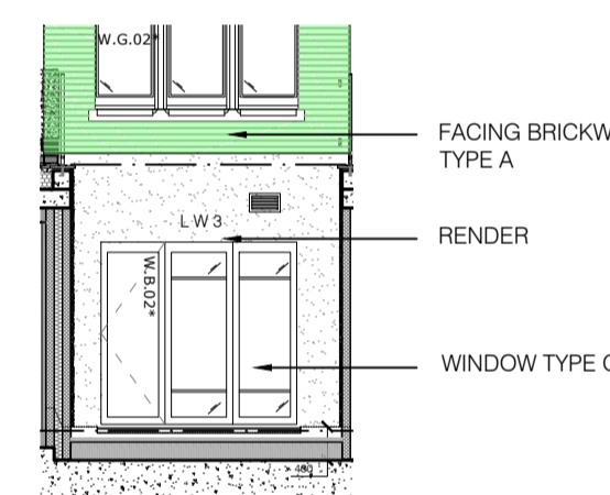
Elevation 3A Scale 1:100
