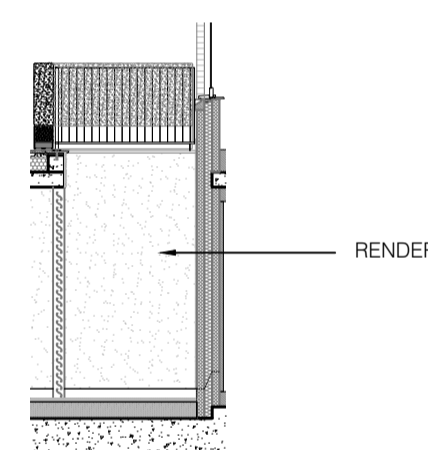
Elevation 3D Scale 1:100
