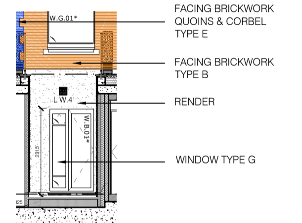
Elevation 4A Scale 1:100
