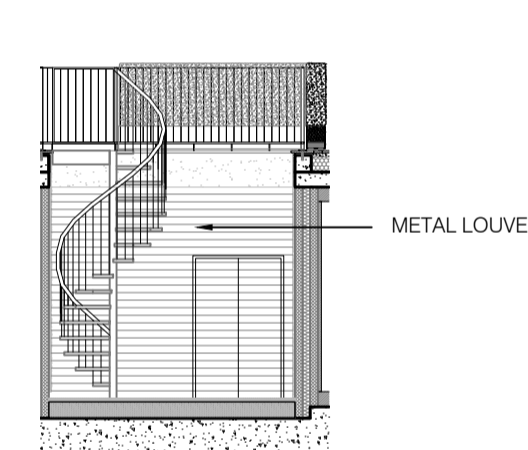
Elevation 3C Scale 1:100
