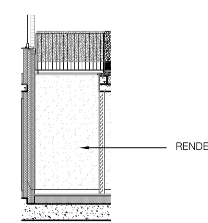
Elevation 2B Scale 1:100
