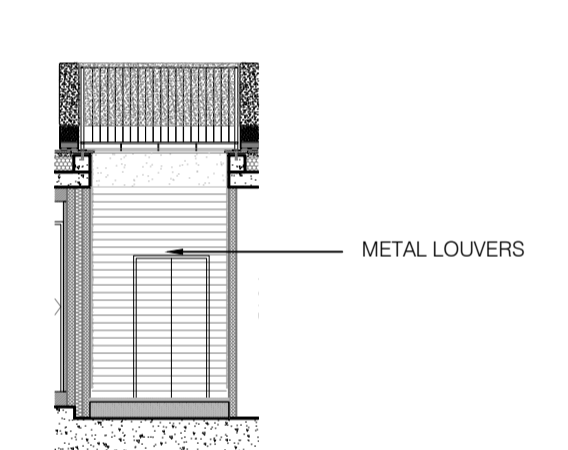
Elevation 4C Scale 1:100
