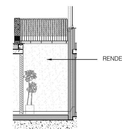
Elevation 4D Scale 1:100
