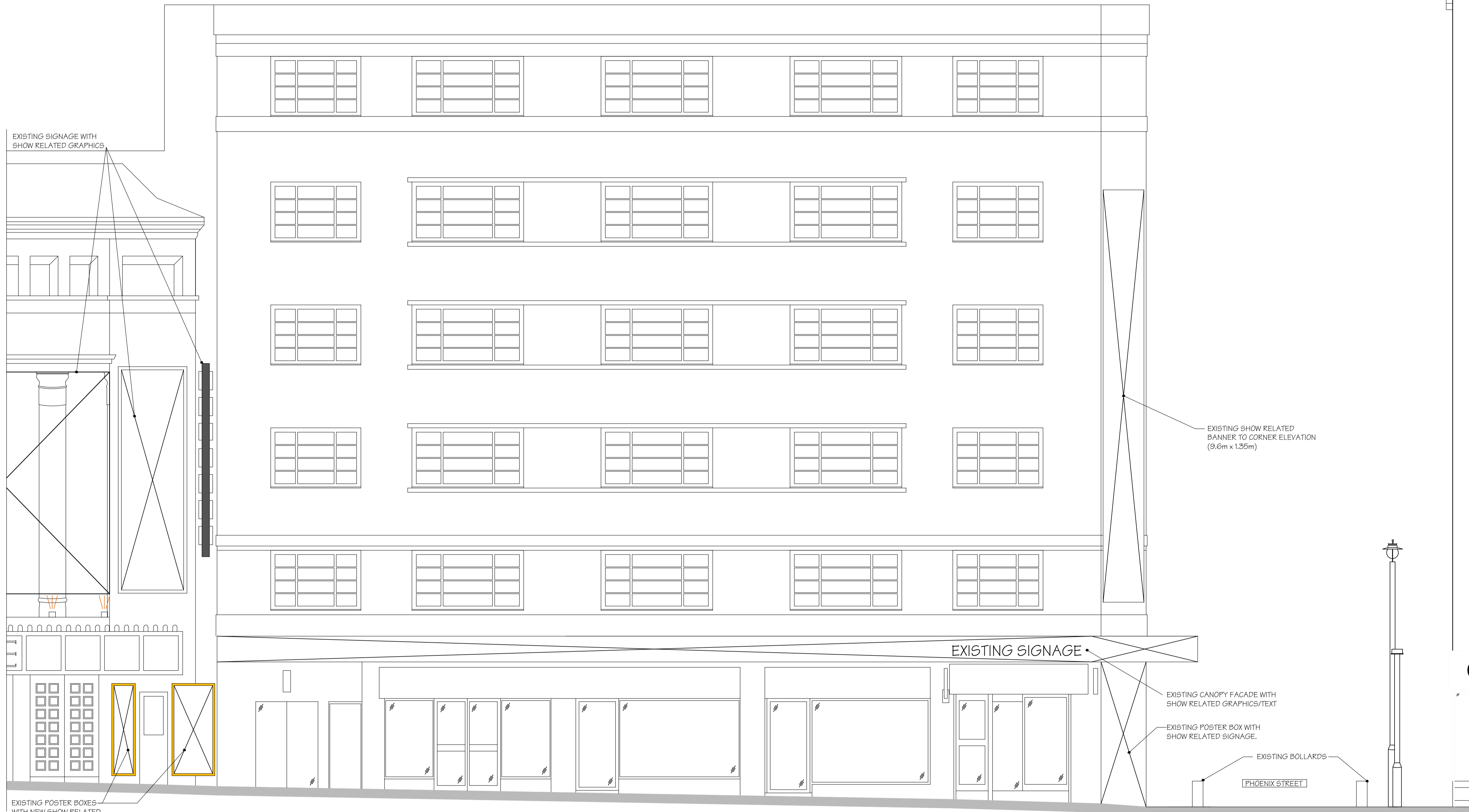
EXISTING CHARING CROSS ROAD ELEVATION (SCALE 1:50 AT A1)
