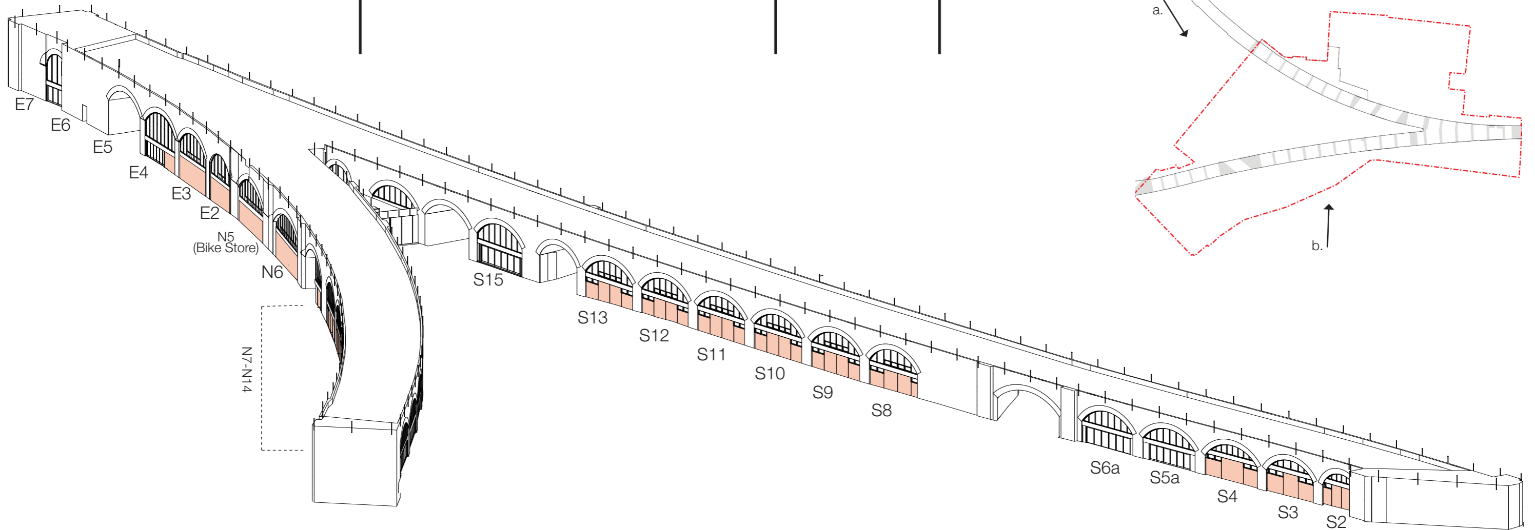
a. Viaduct (south inside)
