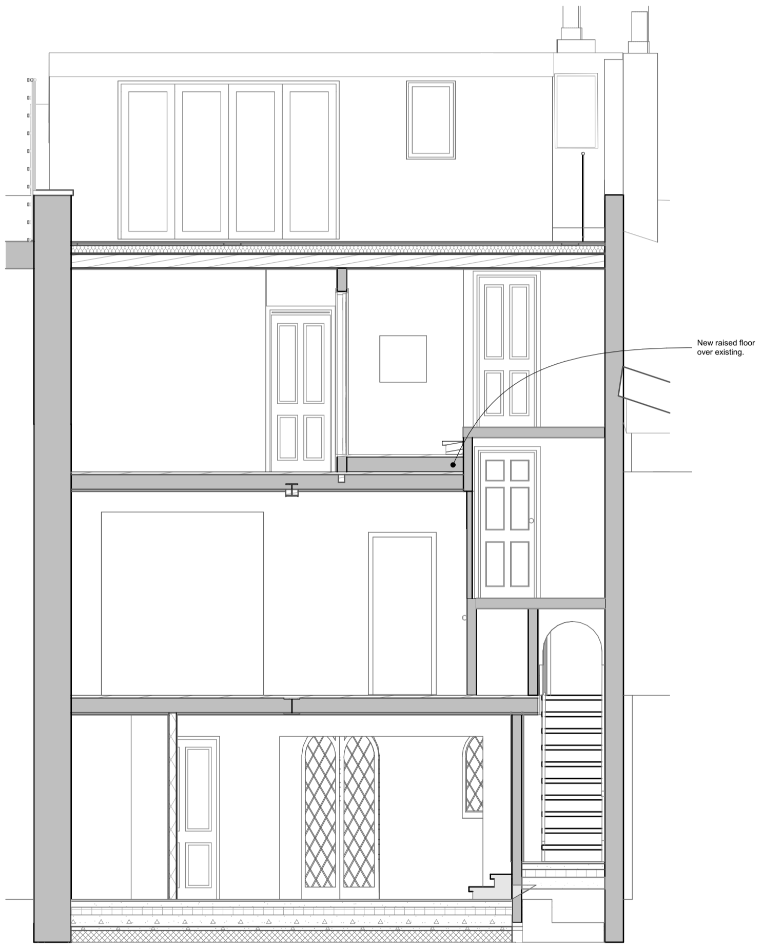
S-10 Building Section 1:50
