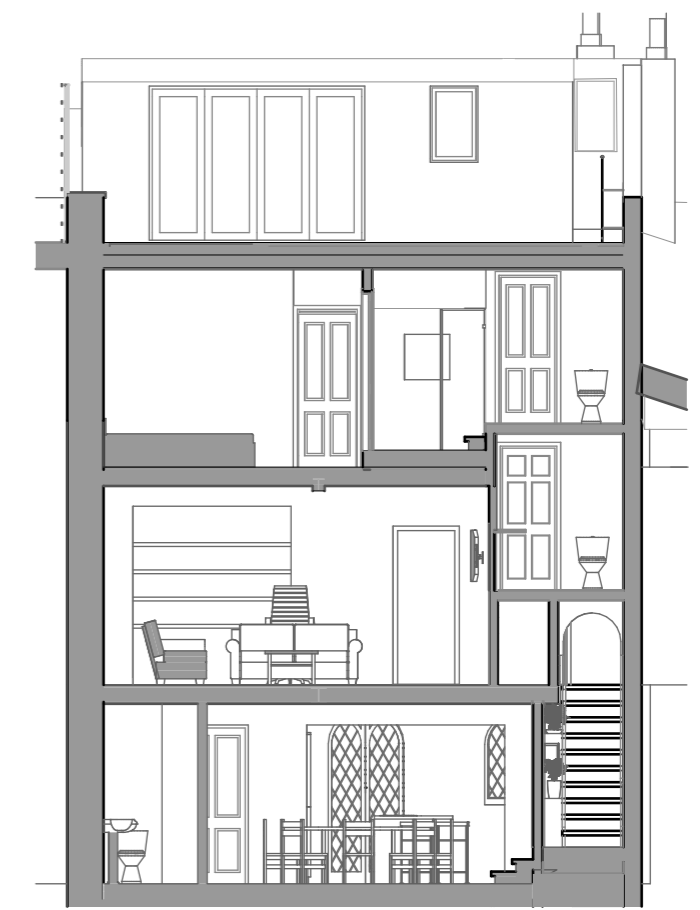
S-10 Building Section 1:100
