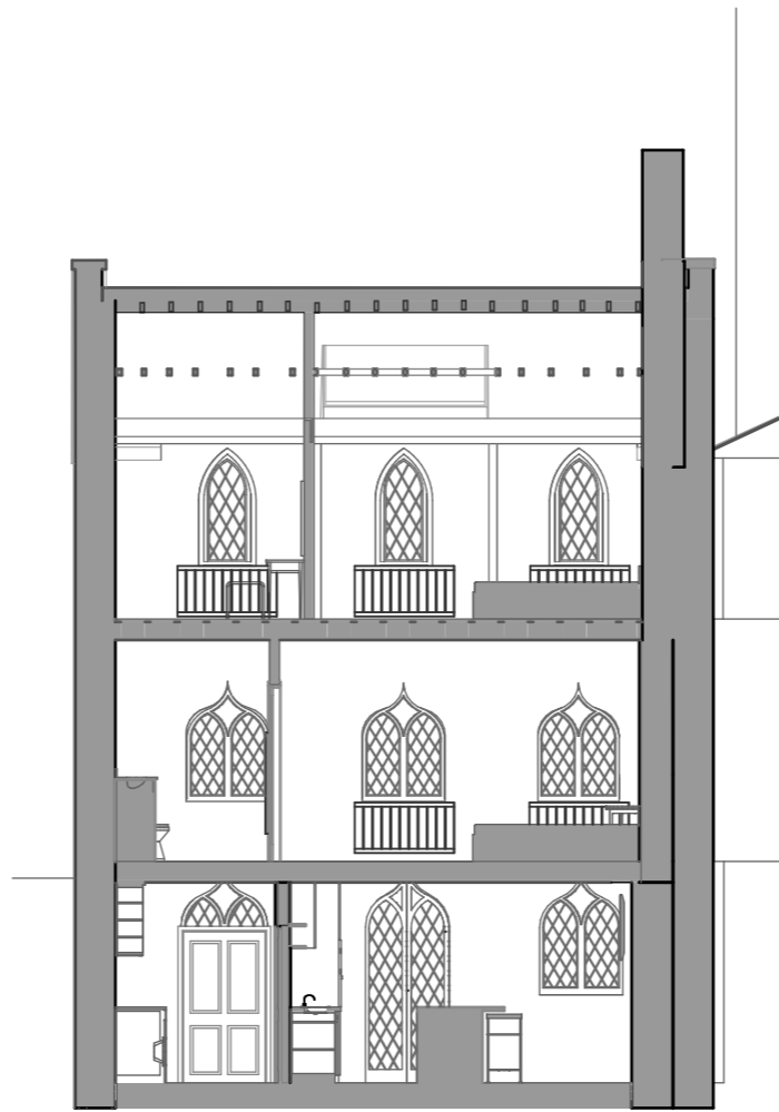
S-08 Building Section 1:100
