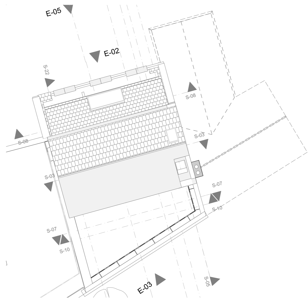
S-32 RF-Proposed Roof Plan 1:100
