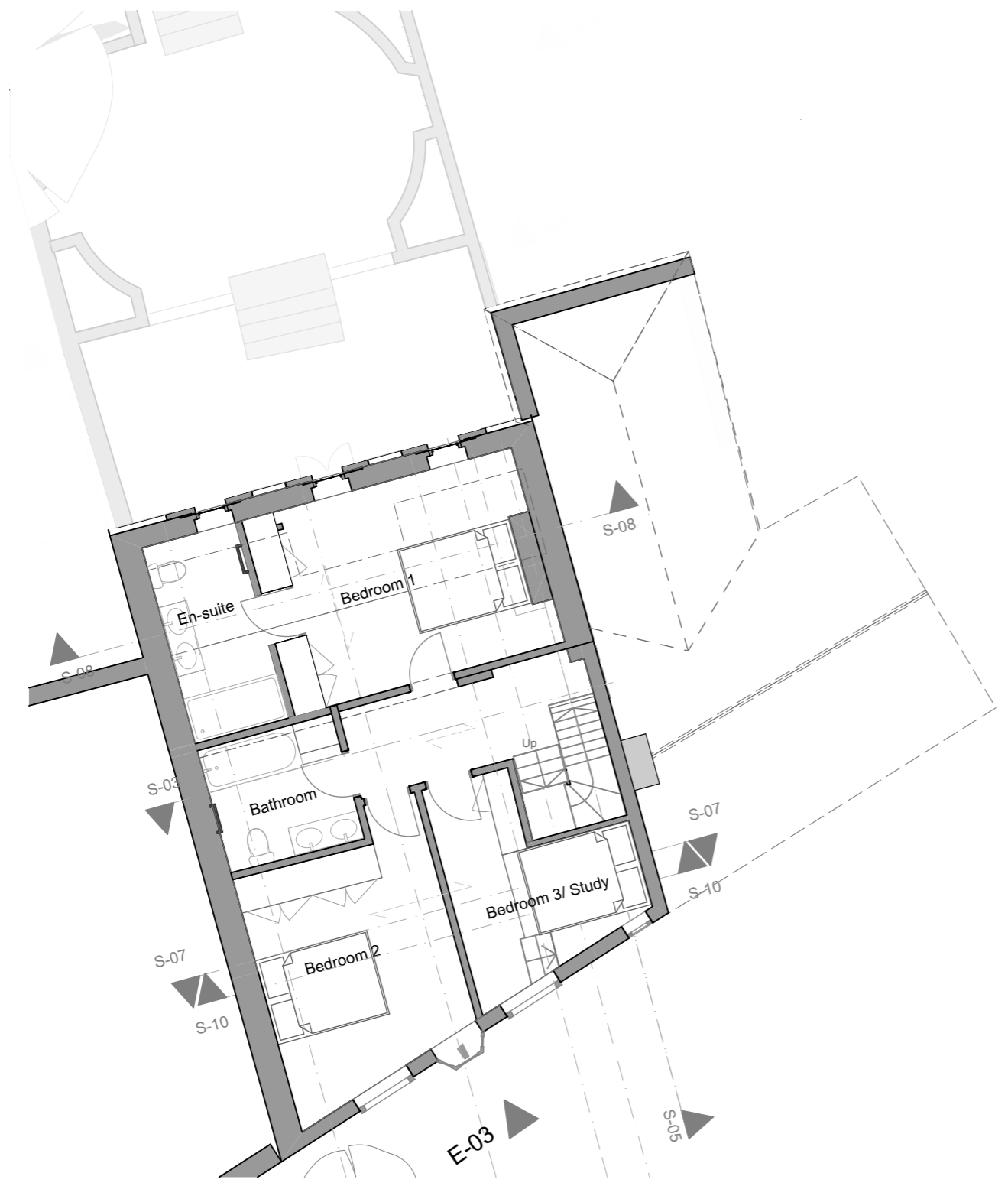
2. 02-Proposed 2FI 1:100
