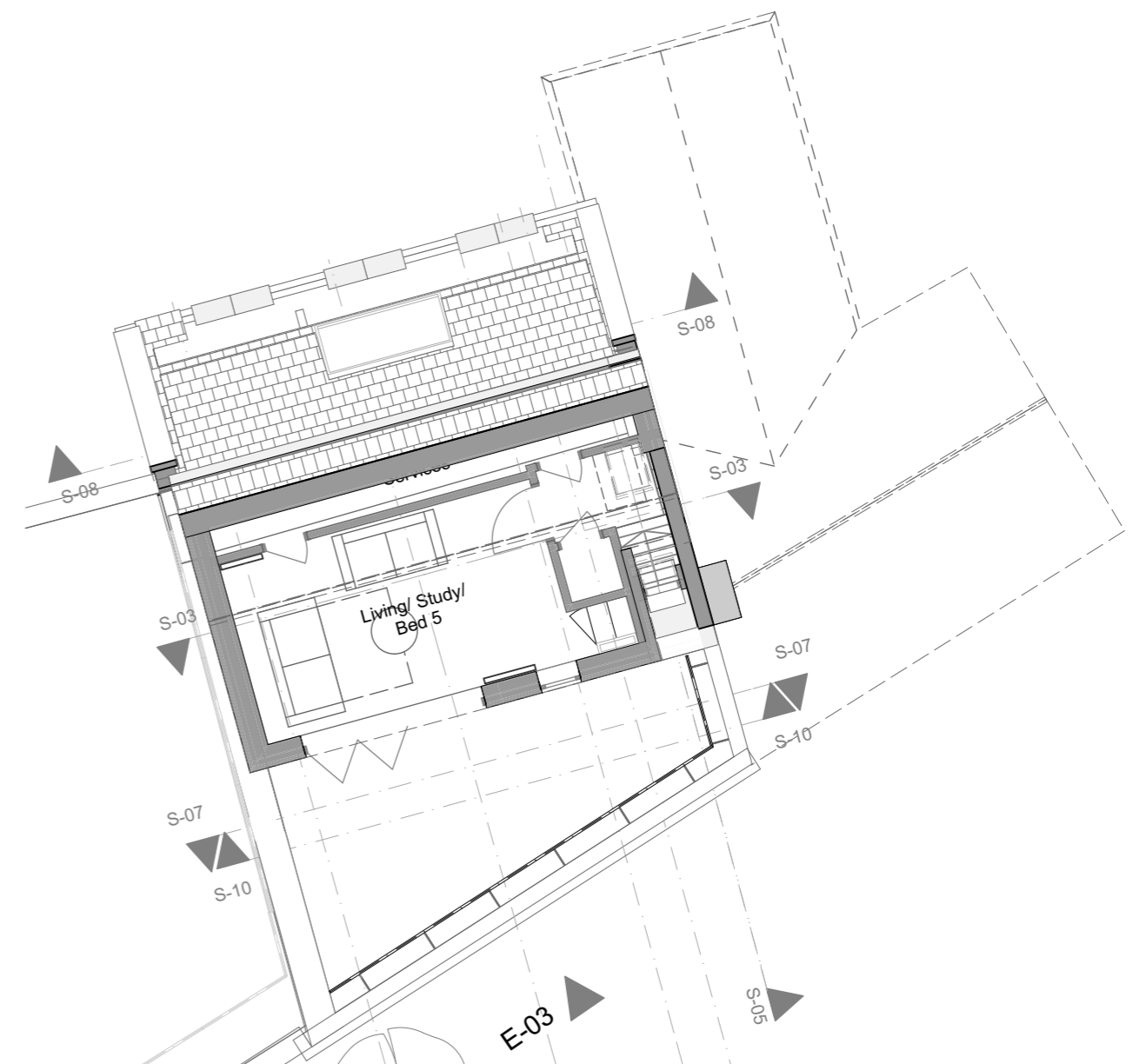
3. RF-Proposed Roof 3F 1:100
