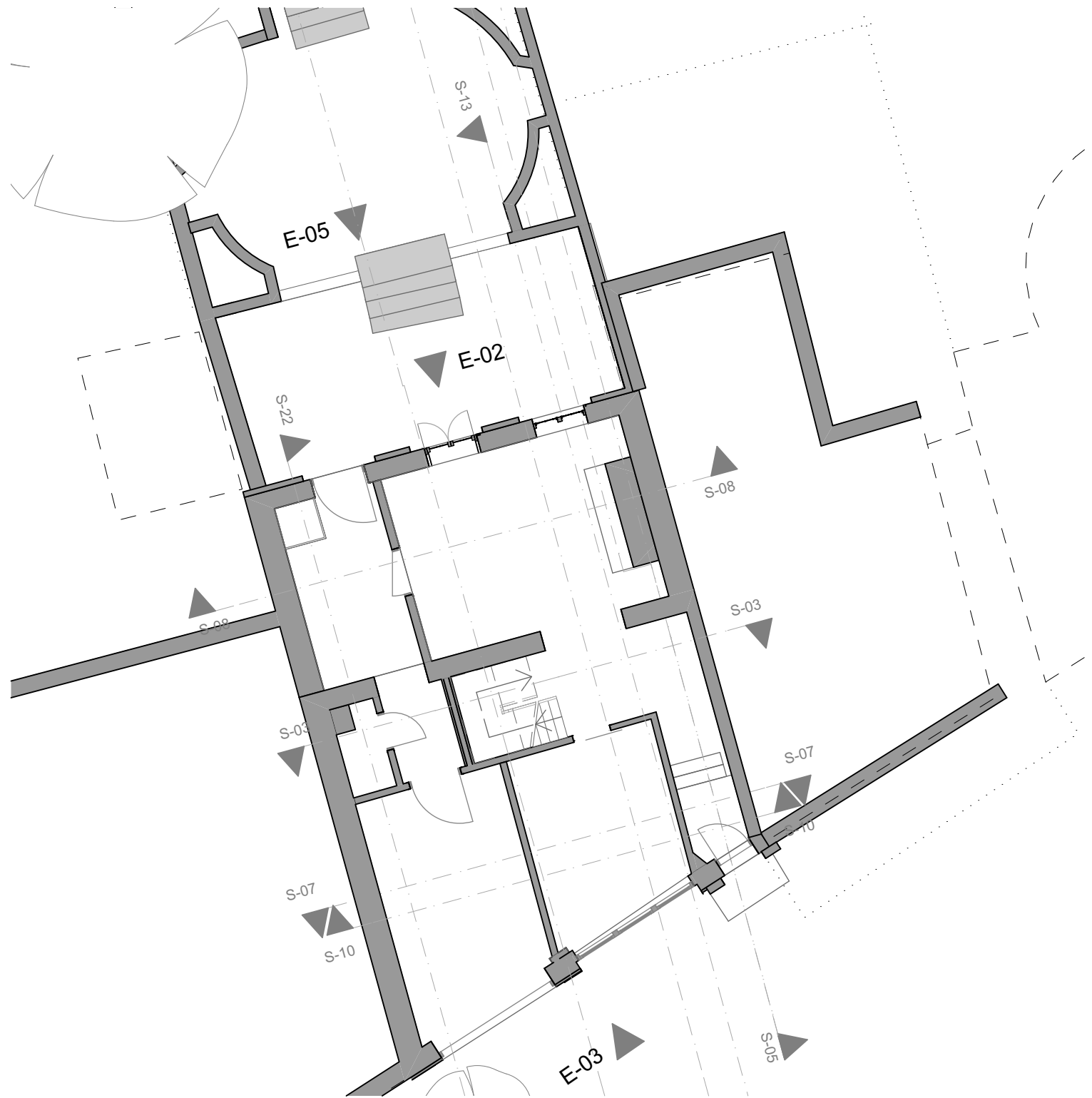
0. GF-Existing GF 1:100
