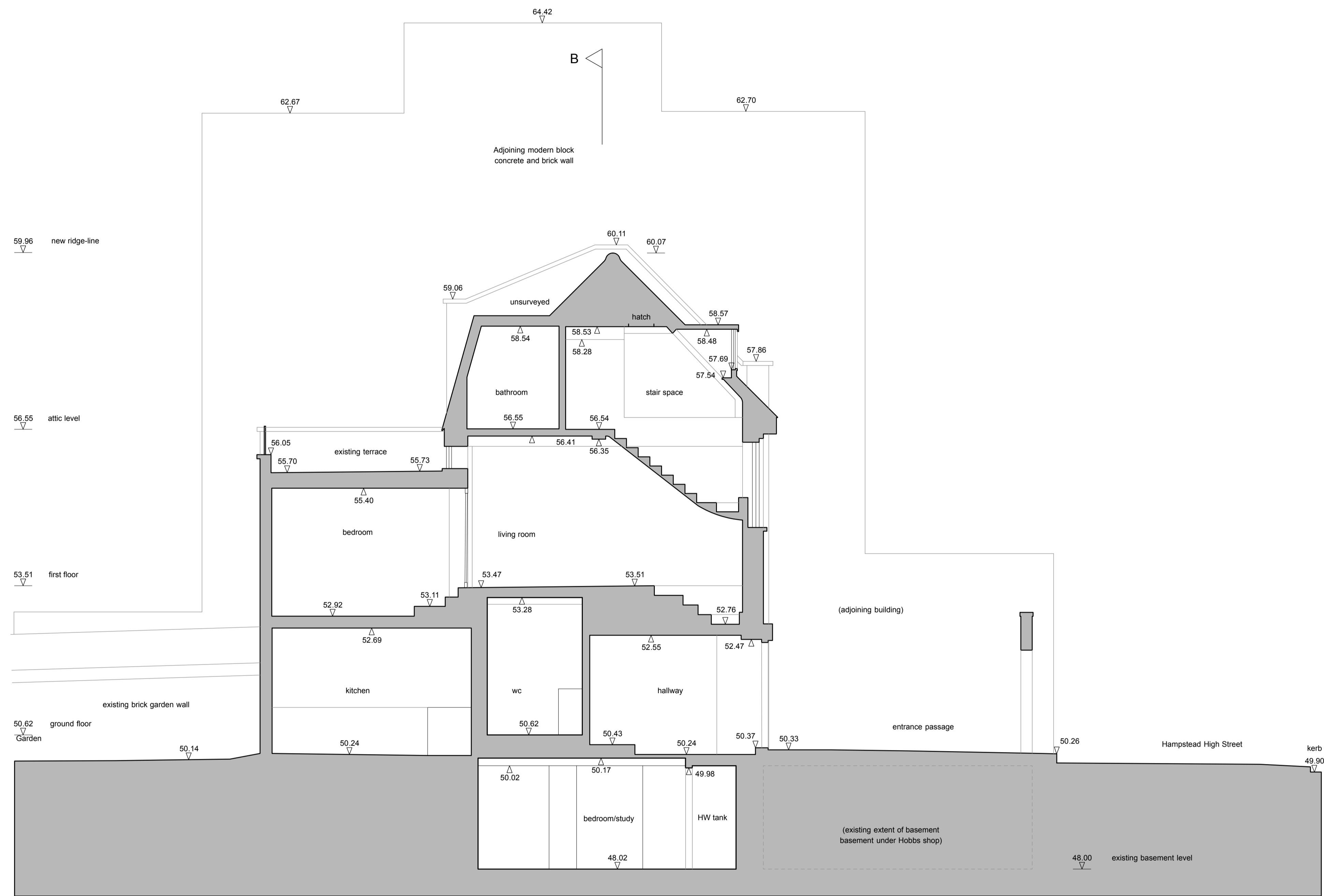
SECTION AA existing survey section
