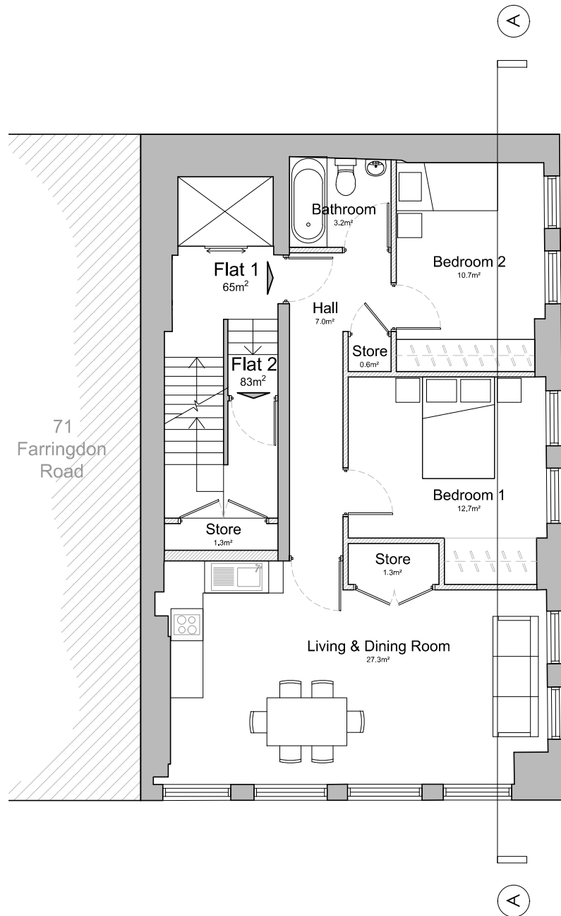
1 Fourth Floor
