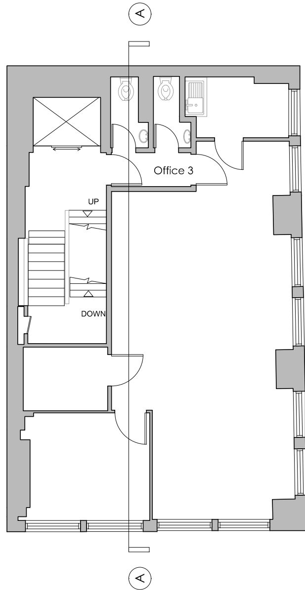
1 Second Floor
