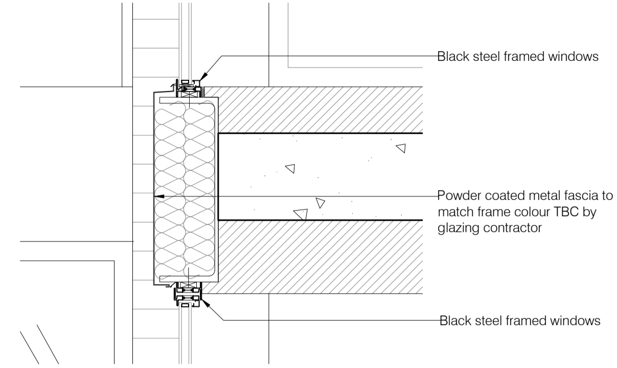
Section C-C Typical metal window head detail Scale 1:10
