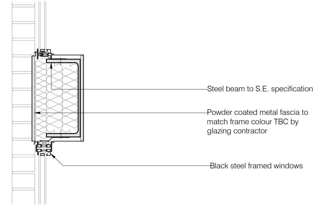
Section B-B Typical window structural transom detail Scale 1:10
