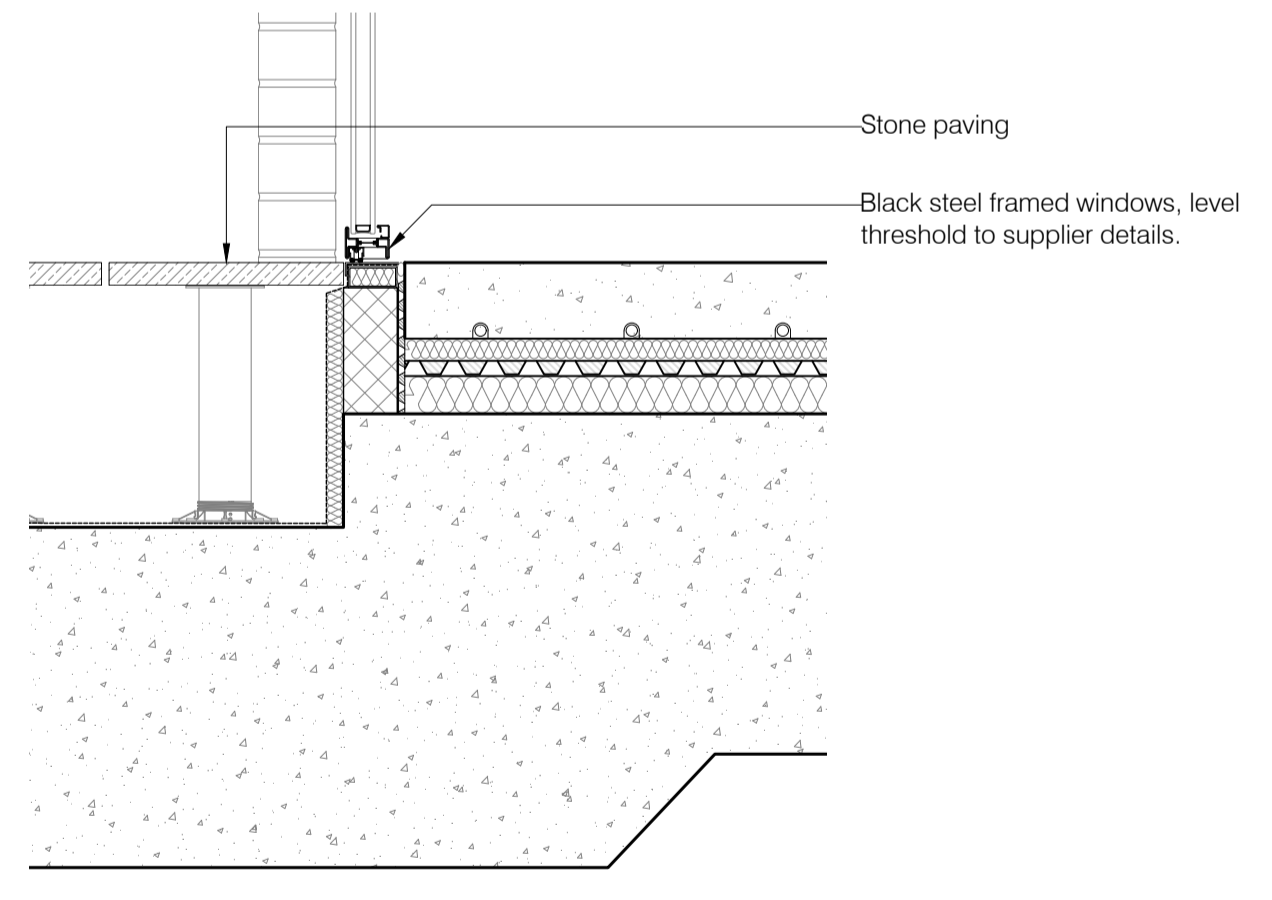
Section G-G Typical metal window sill detail Scale 1:10
