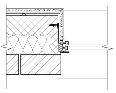
Section A-A Typical jambs detail Scale 1:10
