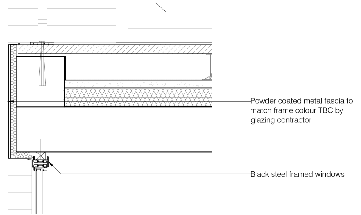
Section D-D Typical metal window head detail Scale 1:10
