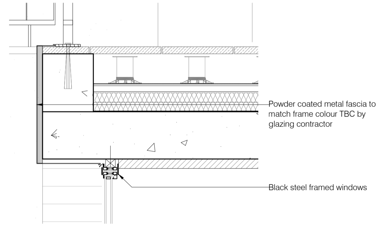
Section E-E Typical metal window head detail Scale 1:10
