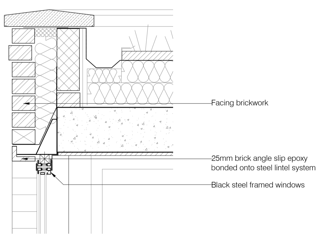
Section F-F Typical metal window head detail Scale 1:10
