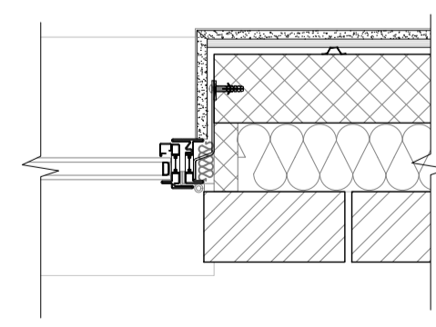
Section A-A Typical jambs detail Scale 1:10
