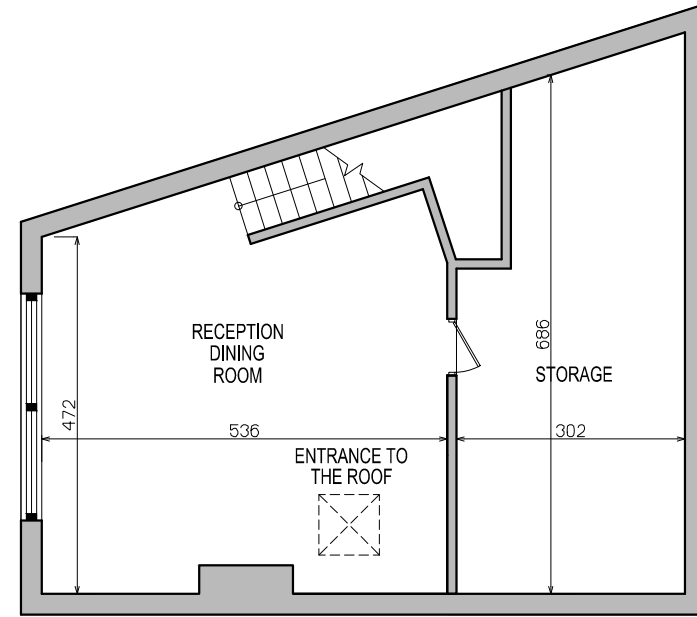
EXISTING THIRD FLOOR
