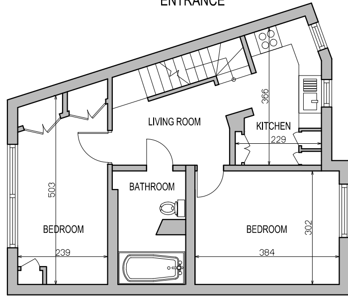
EXISTING SECOND FLOOR
