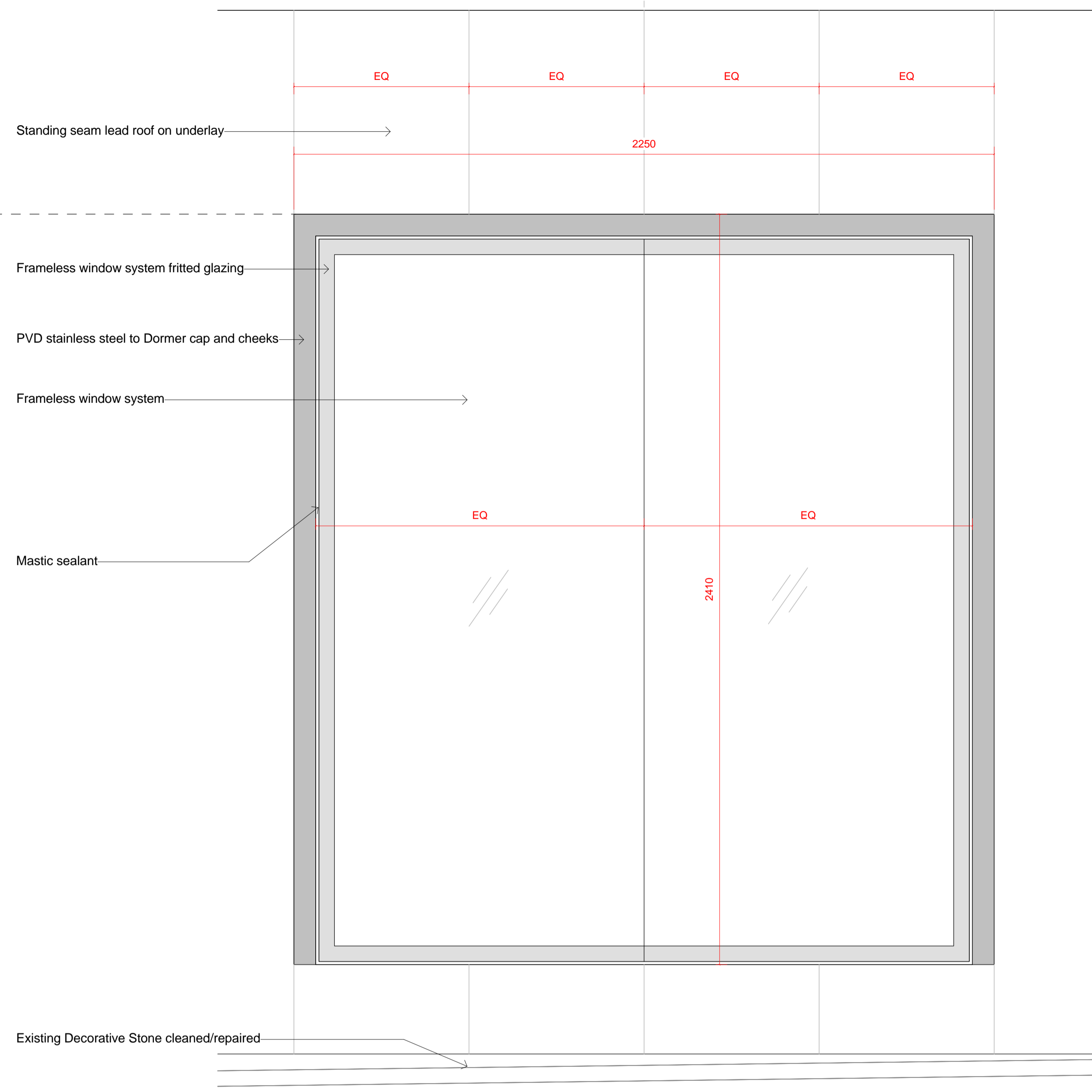
2 25 Denmark Street Dormer Elevation Scale: 1 : 10
