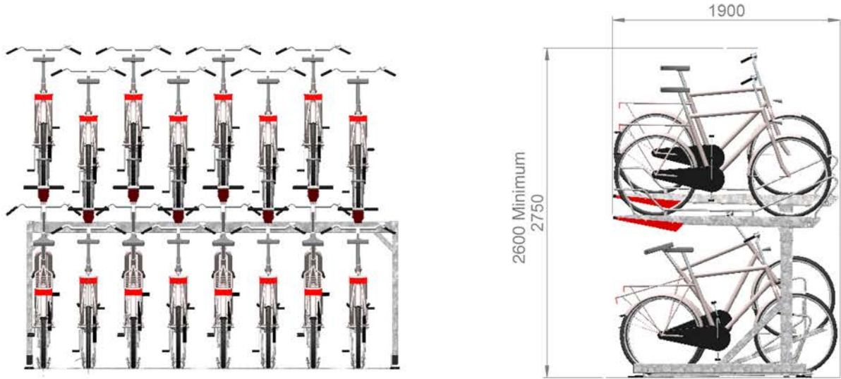
Single sided staggered layout
