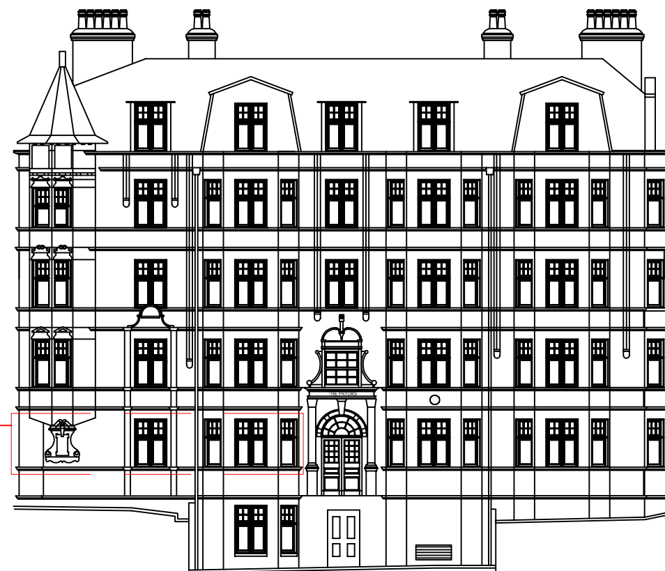
North Elevation
