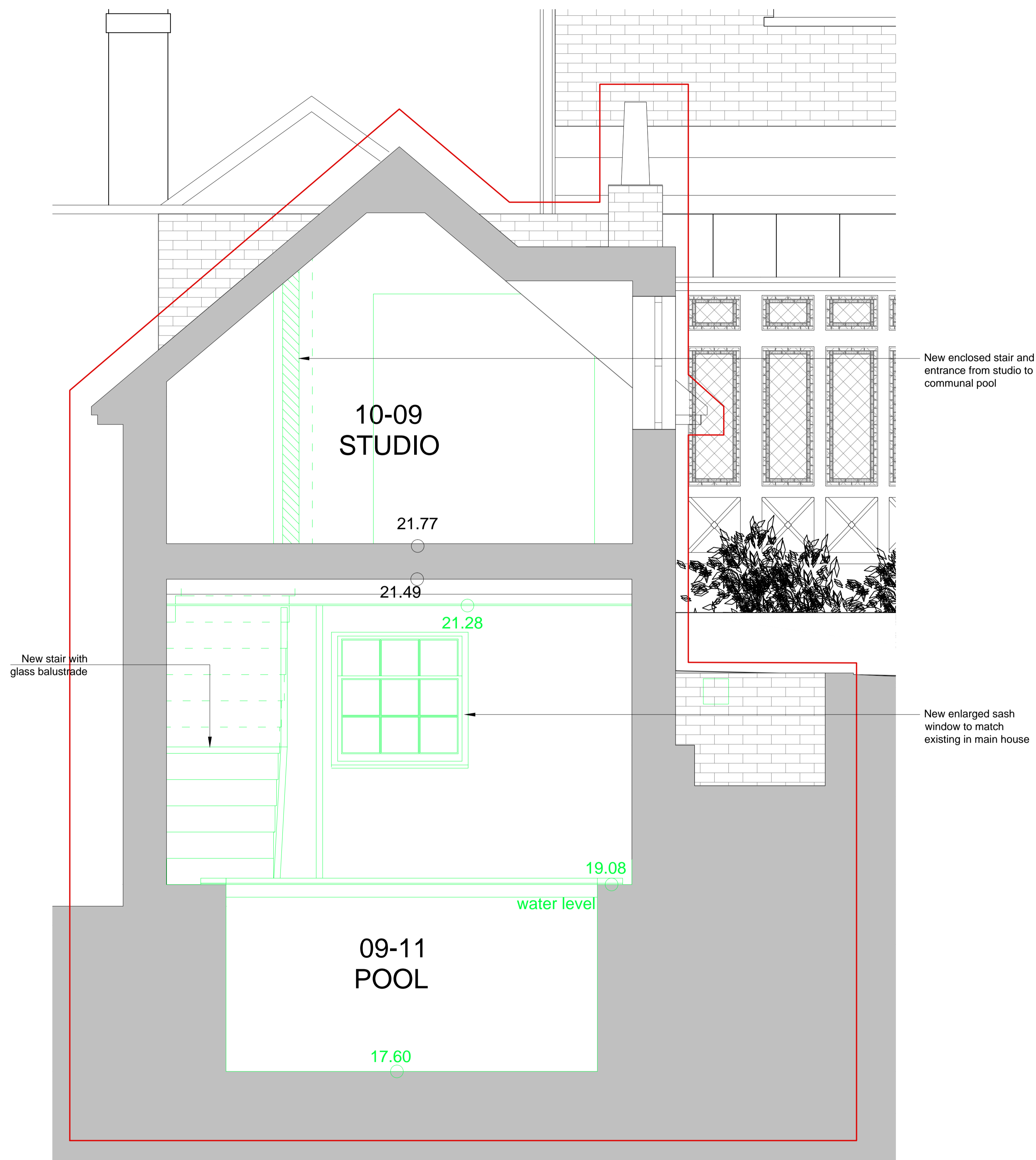
01 PROPOSED POOL - SECTION AA A08 1:40@A3, 1:20@A1
