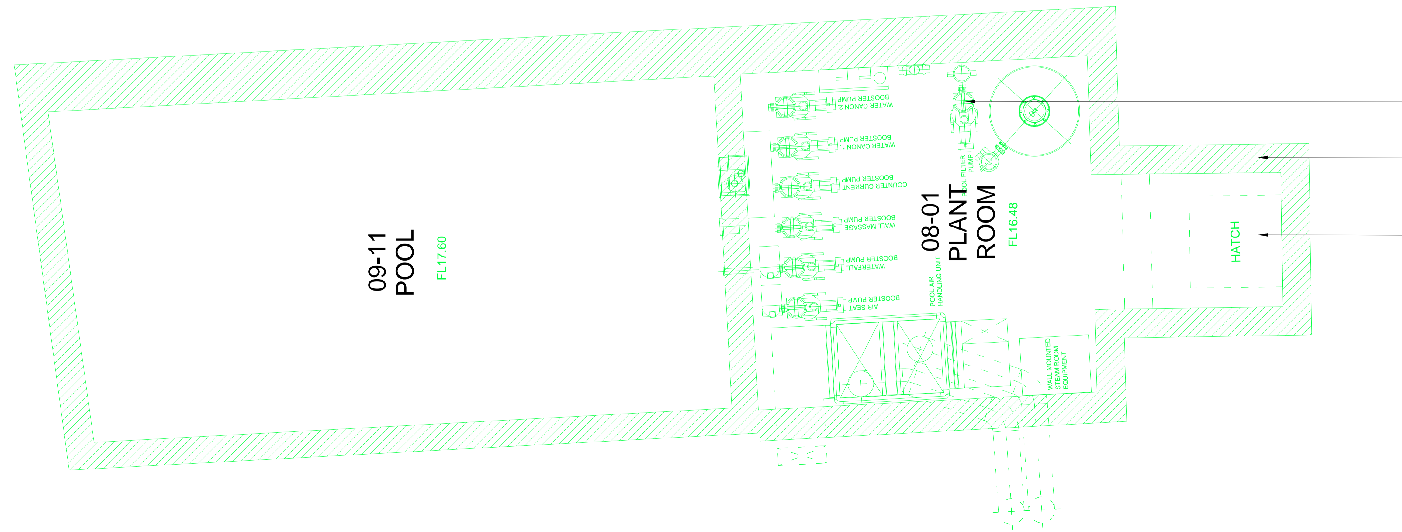
02 PROPOSED PLANT ROOM - PLAN A06 1:40@A3, 1:20@A1
