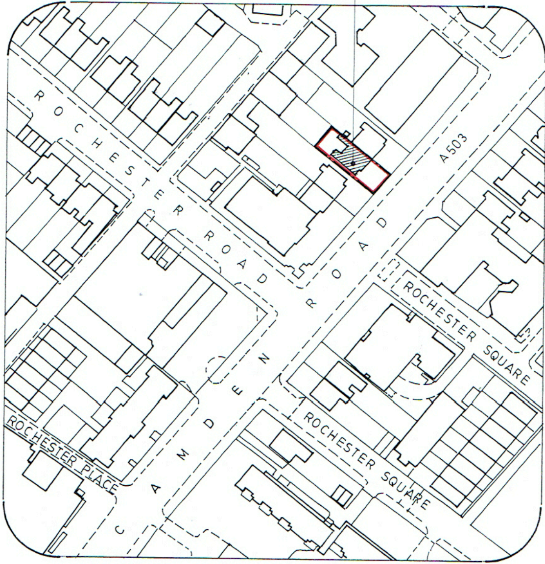
LOCATION PLAN 1:1250
