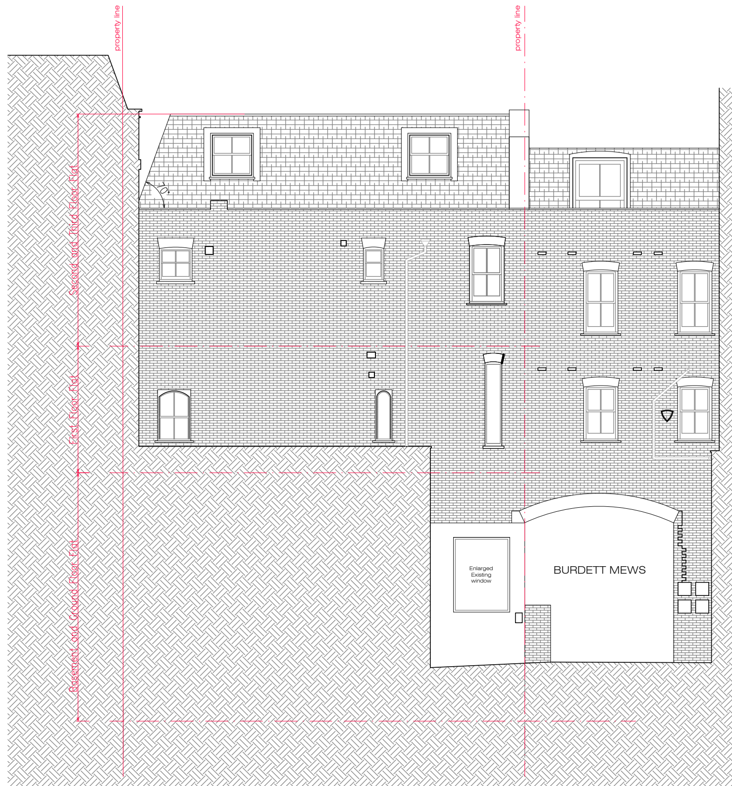
Rear Elevation
