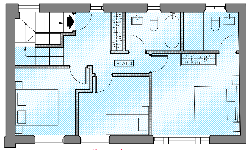
Second Floor
