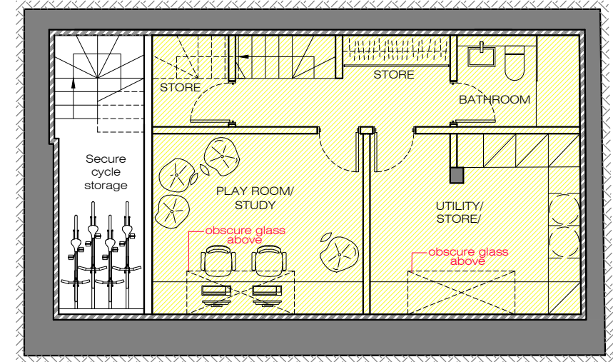
Basement
