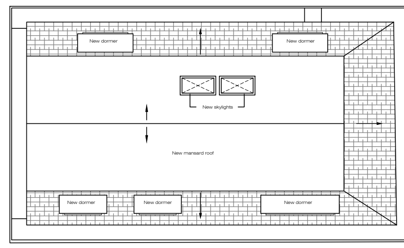
Roof Plan
