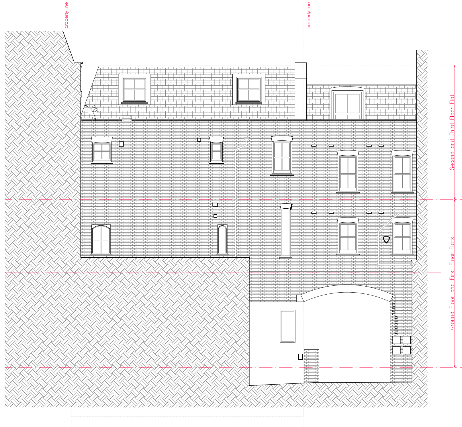
Rear Elevation
