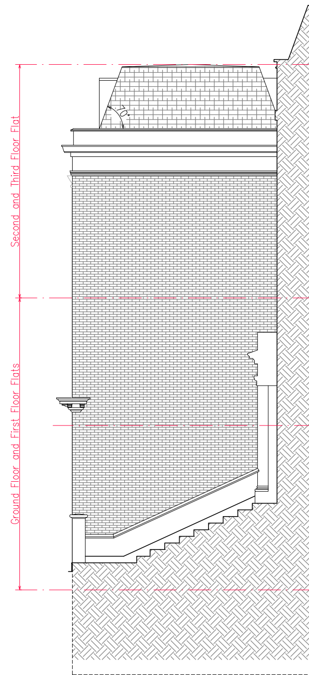
Side Elevation
