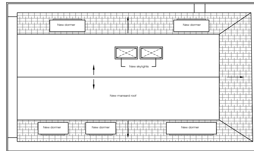
Roof Plan
