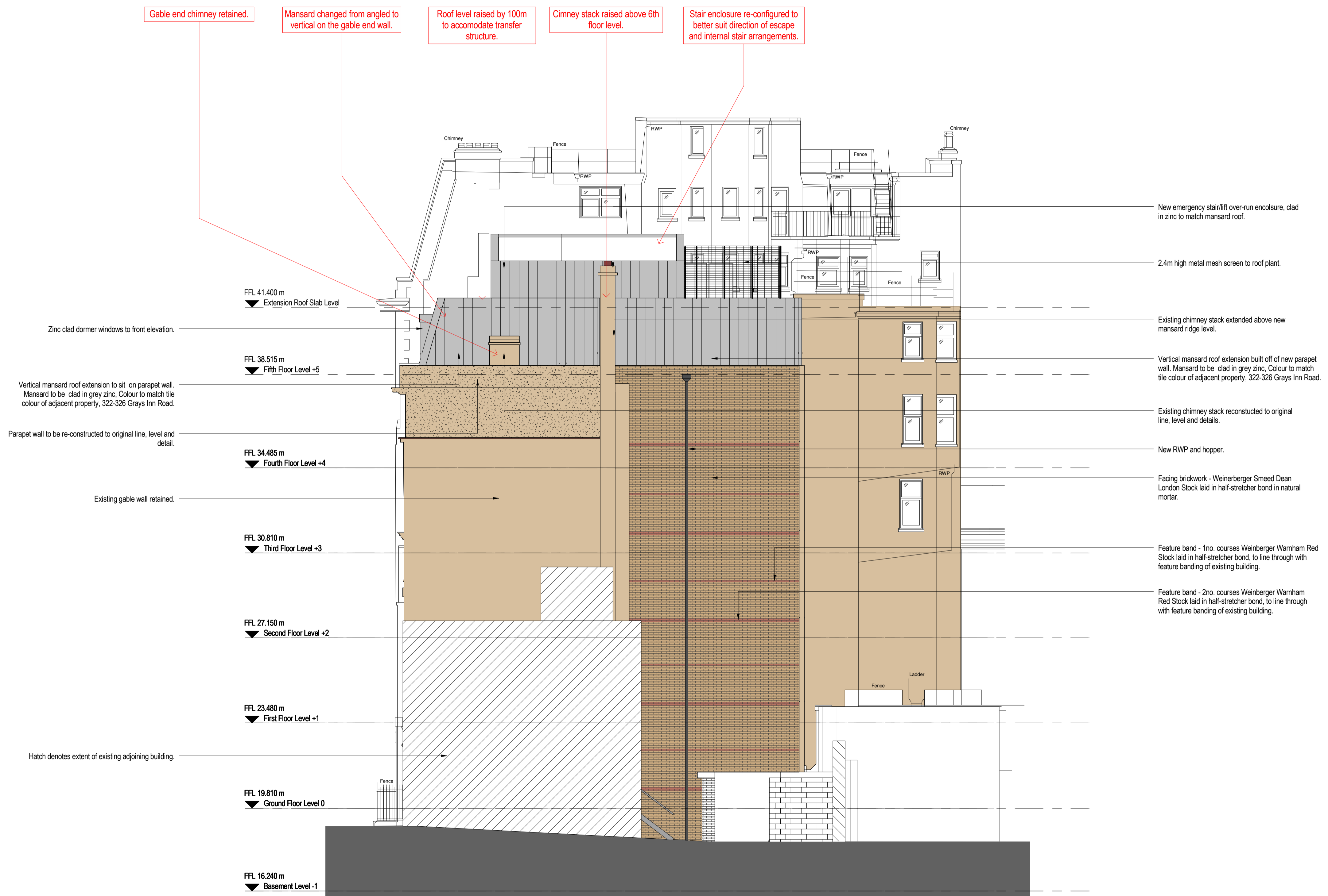
East Elevation 1 : 100
