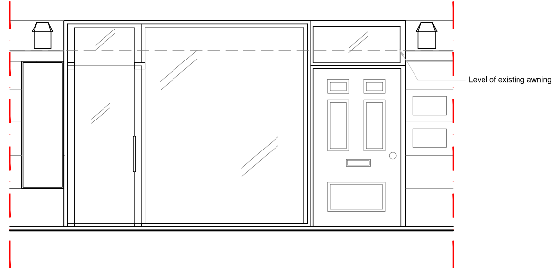
1 Existing Elevation 1:50
